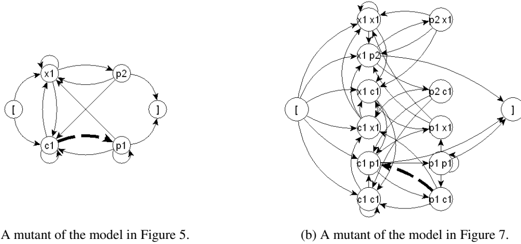
Figure 8. Two mutants generated from morphologically different models (Mutations are shown in boldface dashed lines). [10]
