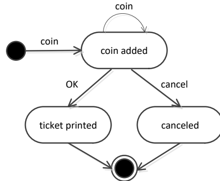
Figure 18. Statechart for simple ticket machine [94]
