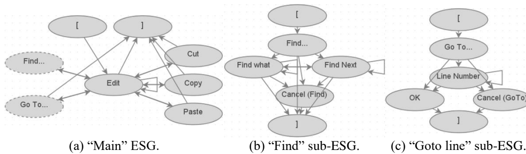
Figure 2. A simplified ESG model of the GUI in Figure 1. [20]
