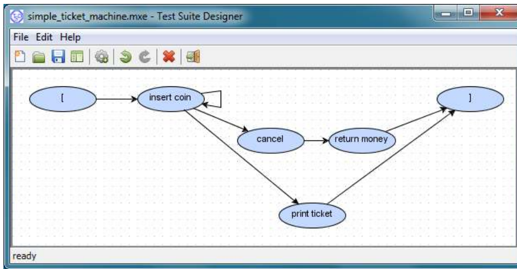
Figure 20. ESG for simple ticket machine in ESG-TSD [96]
