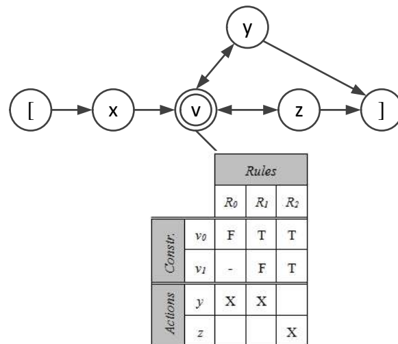
Figure 15. An example of DT-supplemented ESG [73]
