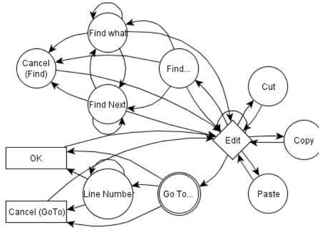
Figure 3. A simplified EFG model of the GUI in Figure 1. [20]
