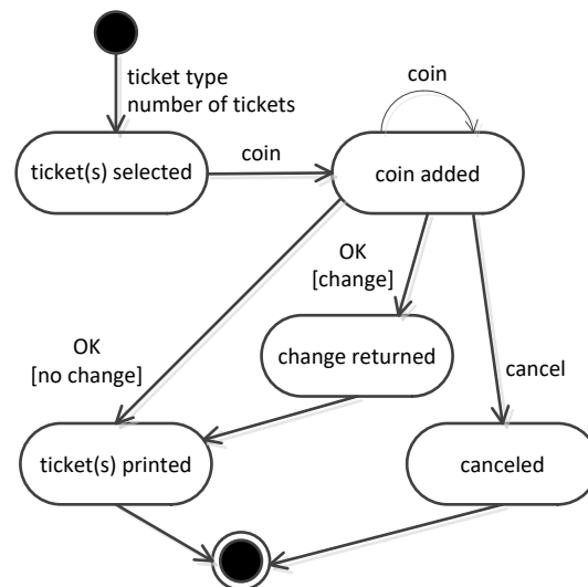
Figure 19. Statechart for complex ticket machine [95]
