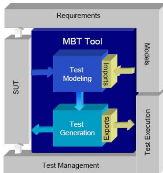
Figure 16: MBTT Categories of Interest
