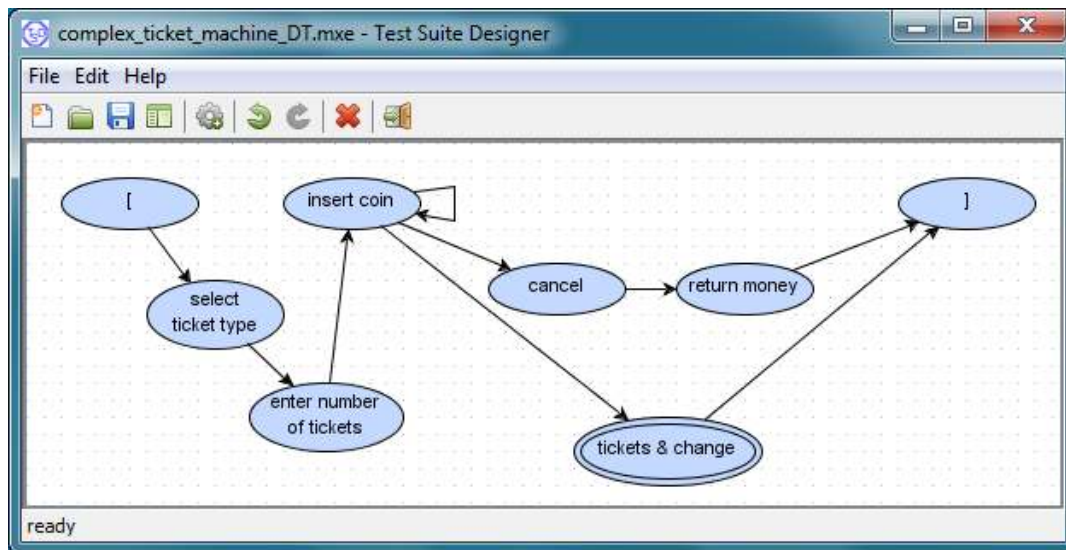
Figure 23. DT- supplemented ESG for complex ticket machine [96]
