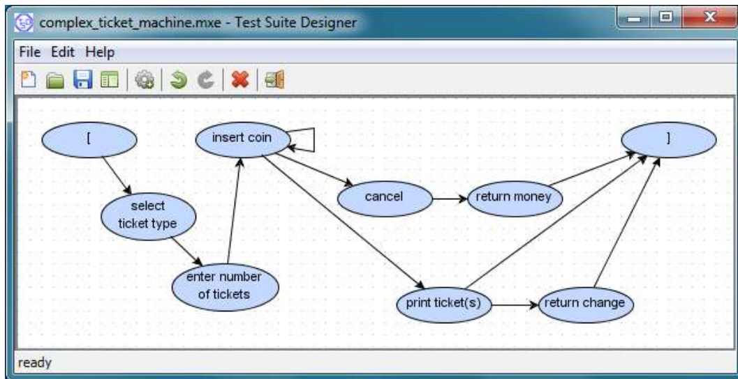
Figure 22. ESG for complex ticket machine [96]
