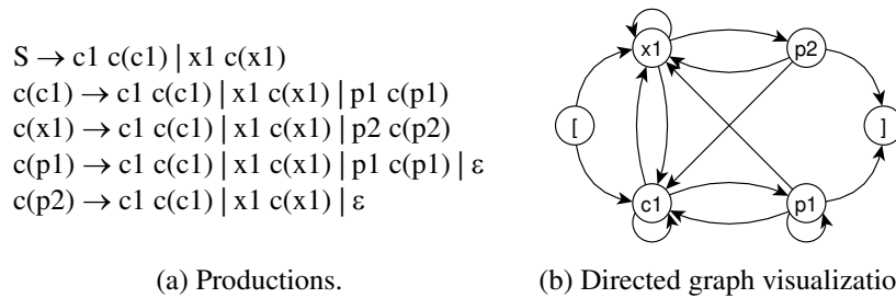
Figure 5. A 1-Reg model. [10]
