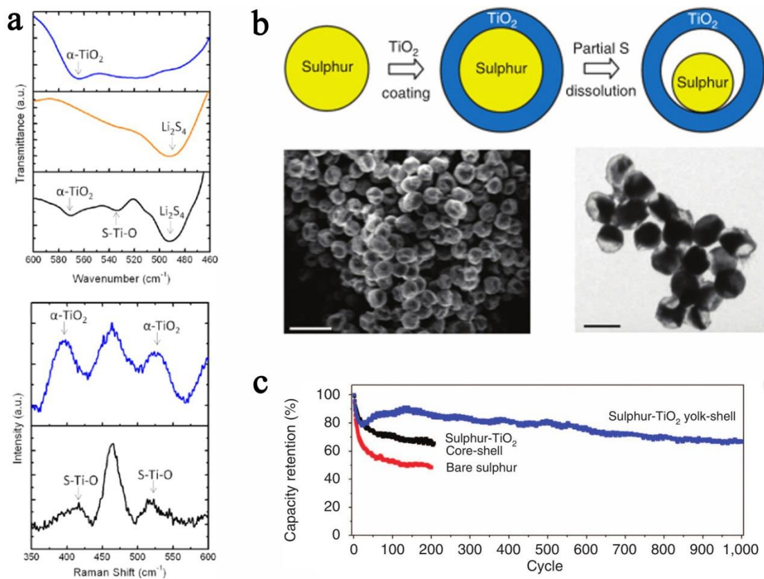
Figure 1. The use of \text{TiO}_2 for Li-S batteries. a) FTIR spectra (top) of \alpha\text{-TiO}_2 , \text{Li}_2\text{S}_4 , and \alpha\text{-TiO}_2/\text{Li}_2\text{S}_4 , and Raman spectra (bottom) of \alpha\text{-TiO}_2 and \alpha\text{-TiO}_2/\text{Li}_2\text{S}_4 . Peaks characteristic of the material are highlighted with arrows. b) Schematic diagram of the synthetic process (top), and SEM and TEM images (bottom) of as-synthesized sulfur-TiO 2 yolk-shell nanostructures. Scale bars, 2 \mu\text{m} and 1 \mu\text{m} for SEM and TEM, respectively. c) Capacity retention of sulfur-TiO 2 yolk-shell nanostructures and control samples cycled at 0.5 C. a) Reproduced with permission. [34] Copyright 2012, American Chemical Society. b,c) Reproduced with permission. [36] Copyright 2013, Nature Publishing Group.
