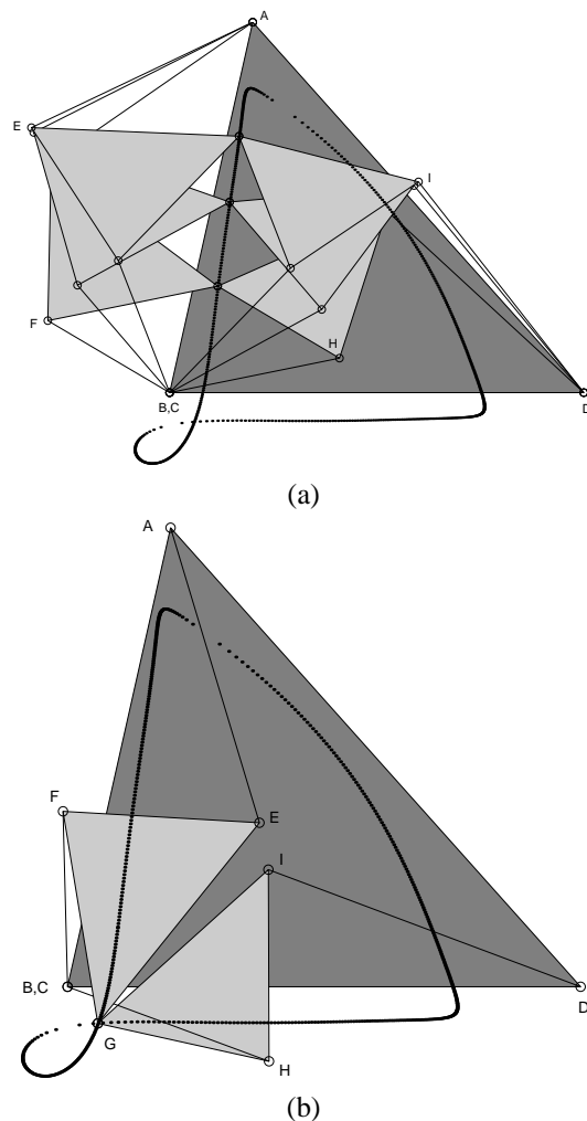
Figure 3. ASSEMBLIES OF A SEVEN-BAR LINKAGE: (A) A SOLUTION CURVE OF DEGREE SIX AND (B) ONE OF SIX ISOLATED SOLUTIONS.
