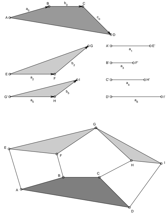
Figure 1. TOP: FIND ALL POSSIBLE ASSEMBLIES OF THESE PIECES INTO A 7-BAR MECHANISM. BOTTOM: ONE SUCH ASSEMBLY.
