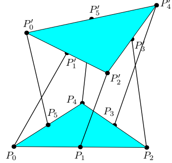
Figure 2. GRIFFIS-DUFFY PLATFORM. BOTH BASE AND ENDPLATE ARE EQUILATERAL TRIANGLES.
