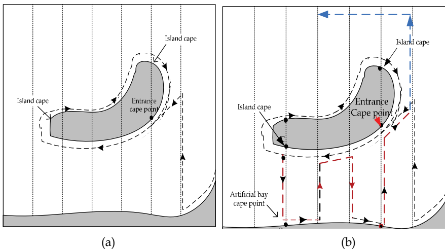
Figure10. Hert's algorithm for non-simply connected area (island)
