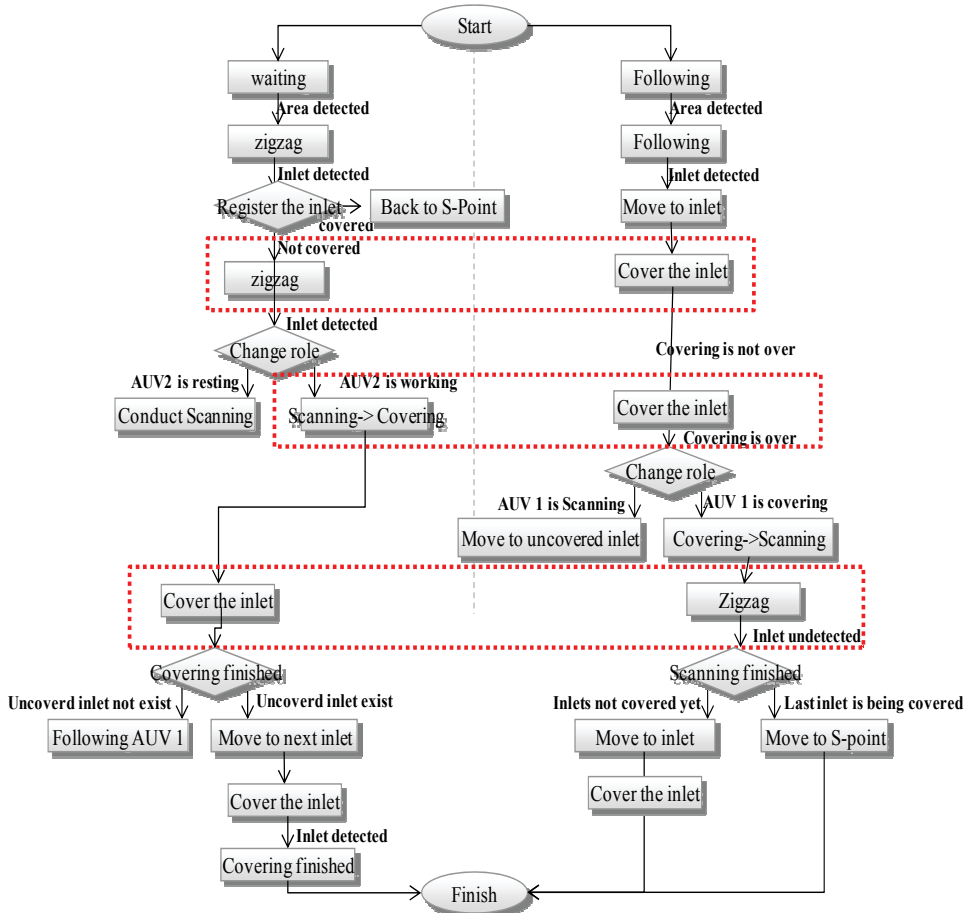
Figure 16. Simulated Multi-AUV work flow
