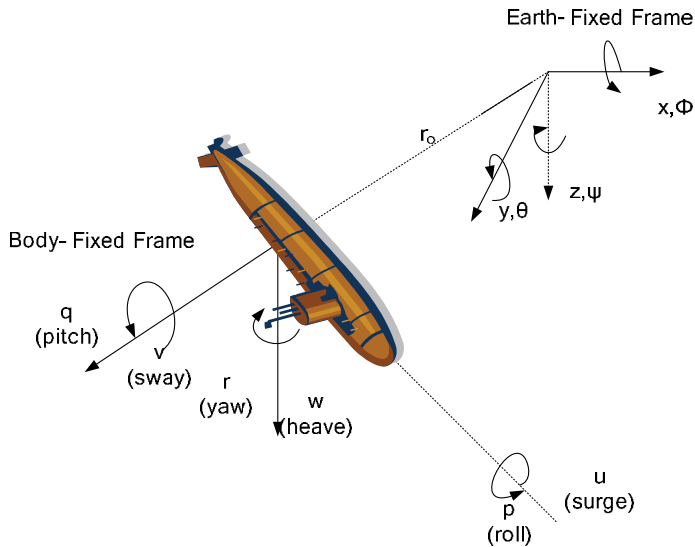
Figure 2. Earth-fixed frame and body-fixed frame for AUV
