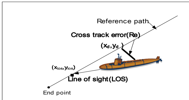
Figure 11. Illustrated cross track error by AUV
