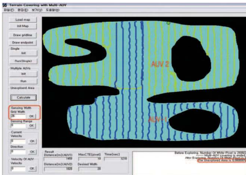
Figure 21. Simulation result of Multi-AUV with EEW
