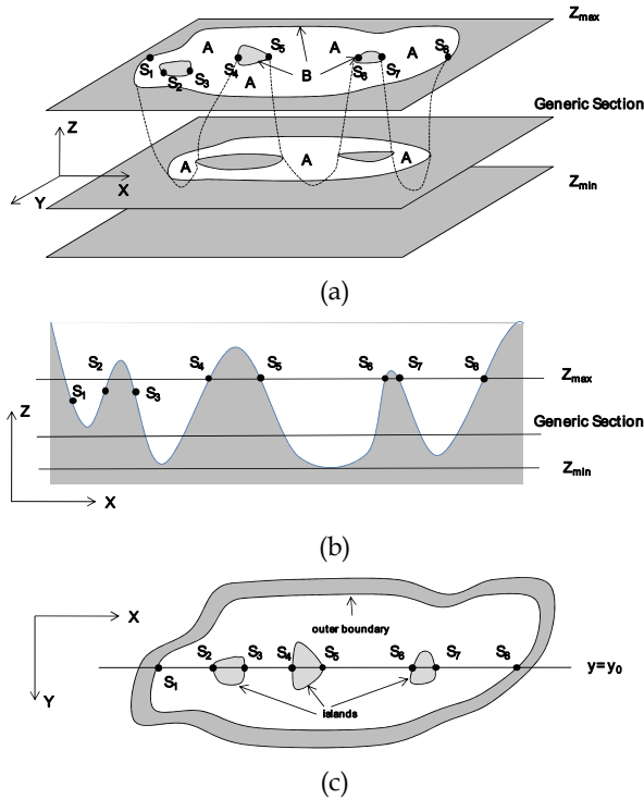
Figure 6. The procedure for converting 3-D underwater environment to 2-D terrain
