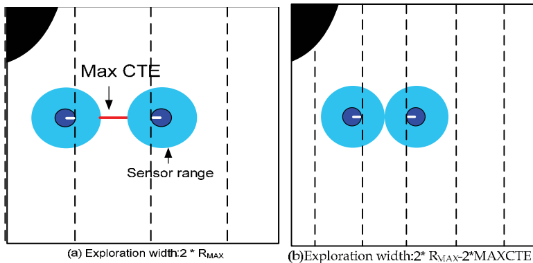
Figure 12. Calculating of EEW using CTE
