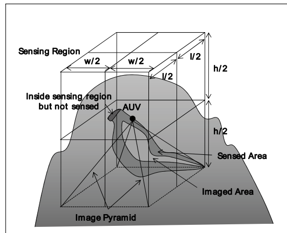
Figure 4. Illustrated AUV sensing model in underwater environment
