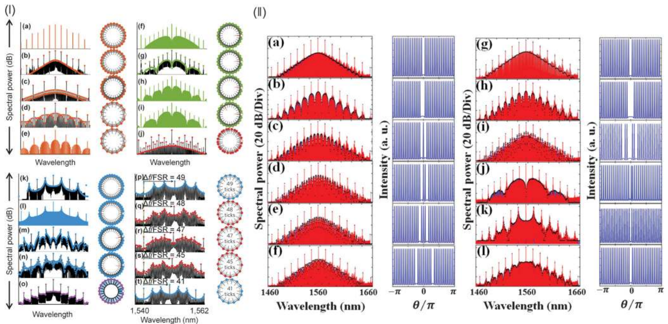
Fig. 13 (I) Soliton crystals in a silica disk resonator. 46 Left panel: measured (in black) and simulated (in color) optical spectra. Right panel: schematic depictions of the corresponding soliton distribution in the resonator with major ticks indicating (expected) soliton location and minor ticks indicating peaks of extended background wave due to mode crossing. (II) Soliton crystals in a high-index doped silica glass microring. 19 Left panel: measured (in red) and simulated (blue solid circles) optical spectra. Right panel: simulated temporal traces exhibiting (expected) soliton distributions of the corresponding soliton crystals. Images are adapted with permission from Refs. 19 and 46.
