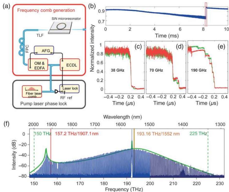
Fig. 4 SMC generation based on power-kicking scheme. (a) Experimental setup of power-kicking scheme. The microresonator is pumped by an external cavity diode laser that is amplified and modulated by an AOM and an EOM. (b) Typical triangular shape of the transmission power while the pump sweeps across a resonance. (c)–(e) Soliton steps of \text{Si}_3\text{N}_4 microcavities with repetition rates of 38, 70, and 190 GHz, respectively. (f) Measured optical spectrum of single SMC covering over 2/3 octave bandwidth. AFG, arbitrary function generator; EDFA, erbium-doped fiber amplifier; FPC, fiber polarization controller; OM, optical modulator; RF, radio frequency; TLF, tapered-lensed fiber. Images are adapted with permission from Ref. 12.
