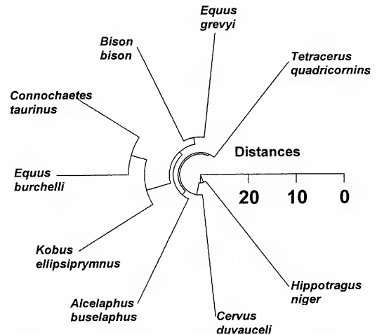
Fig. 14. Cluster tree of the extant grazers.
