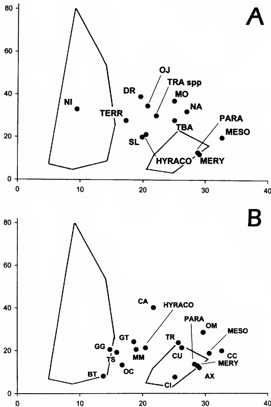
Fig. 17. Microwear in extinct equids showing marked dietary heterogeneity. A. Extinct equids plotted against fruit browsers. Hyracotherium falls near Cephalophus silvicultor . Mesohippus , Parahippus , and Merychippus differ from fruit browsers. B. Extinct equids plotted against selected mixed feeders. Hyracotherium falls near Muntiacus muntjack . Mesohippus , Parahippus , and Merychippus cluster together and are close to Axis axis and Cervus canadensis . There is a shift in the diet from Mesohippus to Parahippus and Merychippus . The latter two tend to graze more (shift by progressive reduction of pits and scratches). Morphospace envelopes of browsers and grazers are included in A and B.
