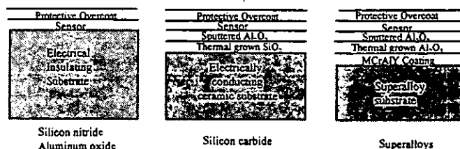
Figure 1. Schematic diagram of thin film sensors on various substrate materials.
