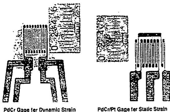
Figure 2. PdCr based thin film strain gauges. (a) dynamic strain gauge and (b) static strain gauge.
