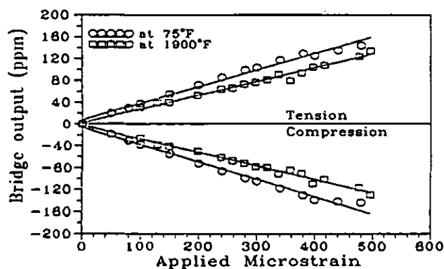
Figure 5. Mechanical response of a PdCr based strain gauge at both room temperature and at 1050^\circ\text{C} ( 1900^\circ\text{F} ).
