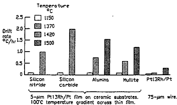
Figure 4. Drift rates for thin film thermocouples compared to that of wire thermocouples.
