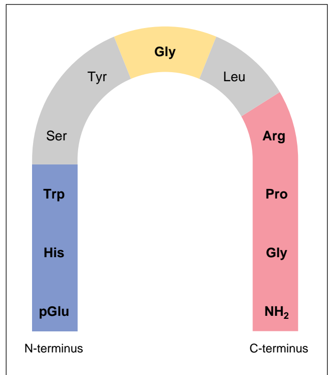
Fig. 2. Structure–activity relationship of GnRH. The amino-terminal residues (blue) have a role in receptor activation, while the achiral Gly residue in position six (yellow) allows GnRH to assume the \beta -turn conformation required for high-affinity interaction with mammalian receptors. The carboxy-terminal residues (pink) are required for specificity and high-affinity binding to the GnRH receptor.
