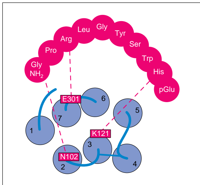
Fig. 4. Diagrammatic representation of GnRH and the mouse GnRH receptor ligand binding pocket. GnRH has been enlarged relative to the receptor, for clarity and to emphasize the relationship of specific residues of GnRH with residues that have been identified in the receptor. The membrane-spanning helices of the receptor are represented by numbered cylinders with connecting extracellular loops shown. The residues that affect ligand binding, Asn 102 , Lys 121 and Glu 301 , are identified. The GnRH residues, GlyNH 2 , Arg 8 and an amino-terminal residue, His 2 , which are affected by mutation of the receptor residues, are indicated by dashed lines.
