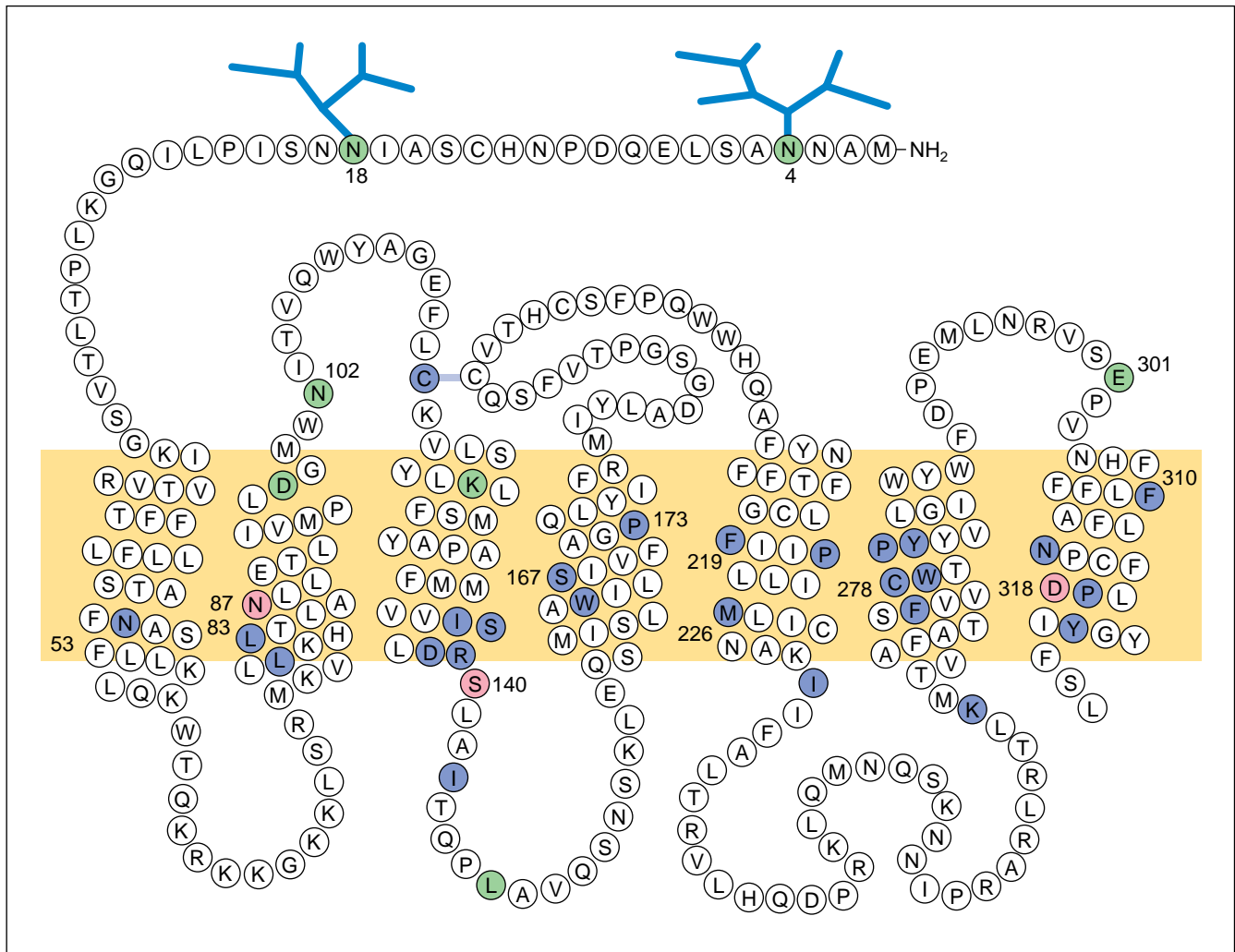
Fig. 3. Two-dimensional representation of the mouse GnRH receptor, a member of the G-protein-coupled family of receptors (GPCRs). Amino acid motifs that are highly conserved throughout the rhodopsin group of GPCRs probably have a role in receptor activation. Indicated by grey circles, they include Asn 53 in helix I; Leu 80 and Leu 83 in helix II; Cys 114 and Ile 135 -Ser-X-Asp-Arg 139 -X-X-Ile 143 in helix III; Trp 164 , Ser 167 and Pro 173 in helix IV; Phe 219 -X-X-Pro 222 , Met 226 and Ile 233 in helix V; Lys 266 and Phe 275 -X-X-Cys-Trp-x-Pro-Tyr 282 in helix VI; Phe 310 , Asn 314 and Pro 319 -X-X-Tyr 322 in helix VII. Some of the residues in positions that are highly conserved among GPCRs are different in the GnRH receptor and provide insight into the structure of GPCRs. These residues are indicated by pink circles: Asn 87 , Ser 140 , Asp 318 . Other residues that affect receptor function and are marked by green circles: Asn 4 , Asn 18 , Asp 98 , Asn 102 , Lys 121 , Leu 147 and Glu 301 .
