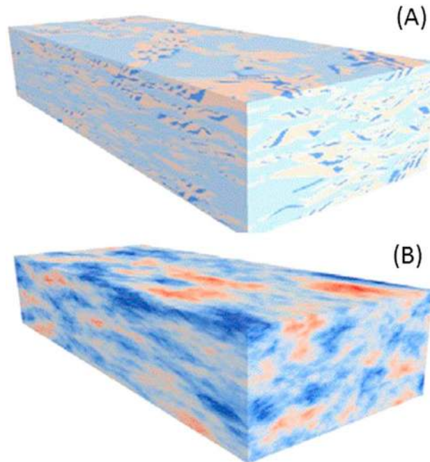
Figure T2.2. Comparison of (a) the three-dimensional heterogeneity patterns generated by the pseudo-genetic method proposed by Pirot et al. [2015a] with (b) a more parsimonious multiGaussian model. The color represents hydraulic conductivity values. The red color corresponds to high values and the dark blue to low values. The domain has a length of 280 m, a width of 110 m, and a thickness of 10.5 m (caption and images modified from Pirot et al. [2015b]).
