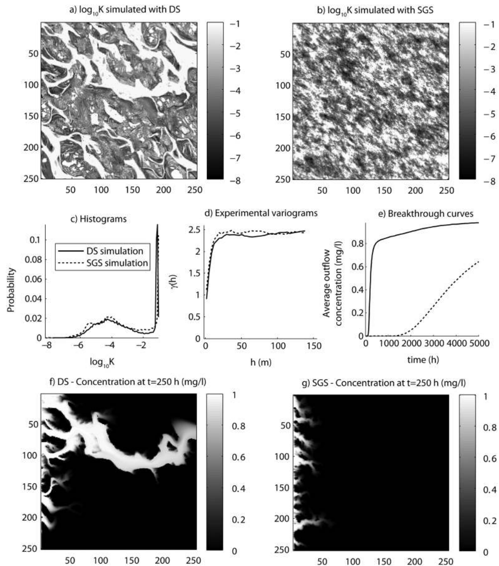
Figure 6. Comparison between Multiple Point Statistics and variogram based geostatistics. (a) One simulation obtained with the Direct Sampling (DS) MPS method. The gray level represents the value of the \log_{10} of the hydraulic conductivity in m/s. (b) One simulation generated using Sequential Gaussian Simulation (SGS). (c) Comparison of histograms of simulated values. (d) Comparison of experimental omnidirectional variograms. (e) Comparison of contaminant breakthrough curves at the outflow boundary. The contaminant is flowing from the left to the right. (f and g) Comparison of the maps of contaminant distribution at t = 250 h, for the case that contaminants were injected along the left boundary (inflow boundary) at t = 0 h. The gray color legend represents the contaminant concentrations. Images and caption text slightly modified after Mariethoz [2009].
