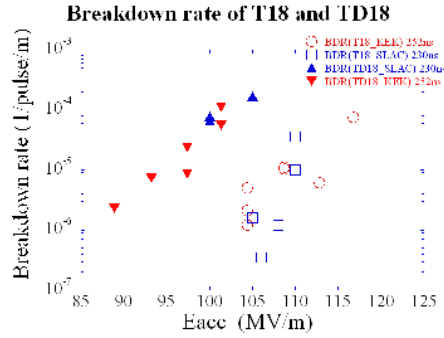
Figure 4: Breakdown rates of T18 (open symbols) and TD18 (solid ones) for pulse widths of 230-250ns. The blue symbols are SLAC results while red ones are KEK results.
