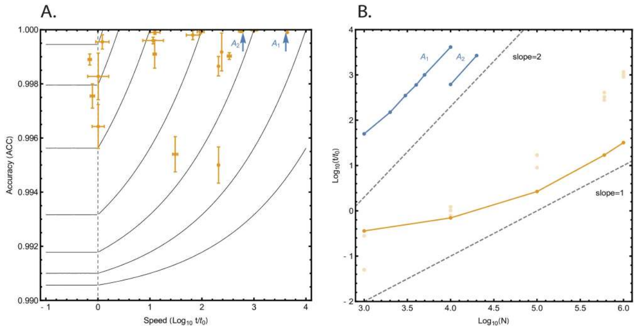
Fig 2. Antibody challenge outcomes. (A): Evaluation metric used for Antibody Clustering as a function of time ( t measured in units of t_0 = 100\text{ms} ) and accuracy ( ACC ), as determined during the competition. Solutions lying on the isocurves are considered equivalent in quality, as defined by the evaluation metric. Data points correspond to average performance based on up to four 10K test sets (failed test cases excluded). Also shown is the benchmark algorithm implemented in Python ( A_1 ) and C++ ( A_2 ); note that benchmark algorithms A_1 and A_2 have perfect accuracy ( ACC equal to unity). (B): Effective computational cost (excluding I/O) on a single core as a function of test set size N for Antibody Clustering ( t measured in units of t_0 = 100\text{ms} ). Dashed lines indicate linear and quadratic scaling behaviors. Results are shown for the benchmark algorithms ( A_1 and A_2 ) and the top four performing solutions (top solution indicated by solid line and darker data points). The benchmark algorithms exhibit quadratic scaling behavior with test set size, whereas the top algorithm exhibits better than quadratic scaling behavior within the regime considered. The best performance over the entire range of N can be achieved using an ensemble of solutions selected based upon whether the test set size is either below or above the crossover value at approximately N \sim O(10^4) .
