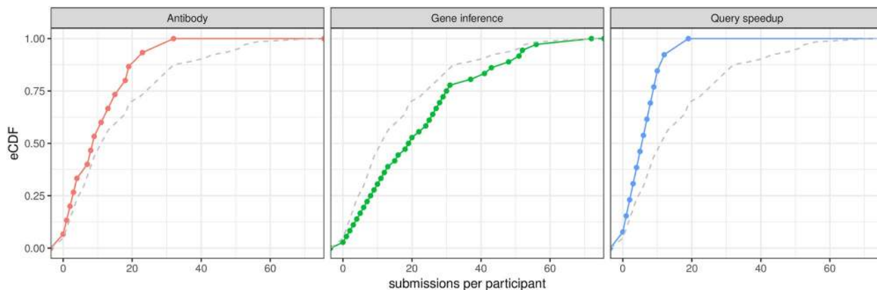
Fig 1. Submissions per participant. Empirical CDF of submissions per participant for the Antibody (left panel), Gene inference (middle panel), and Query speedup (right panel) competitions. Each panel also reports the empirical CDF of the submissions per participant based on the aggregated data for the three competitions (dashed curve).
