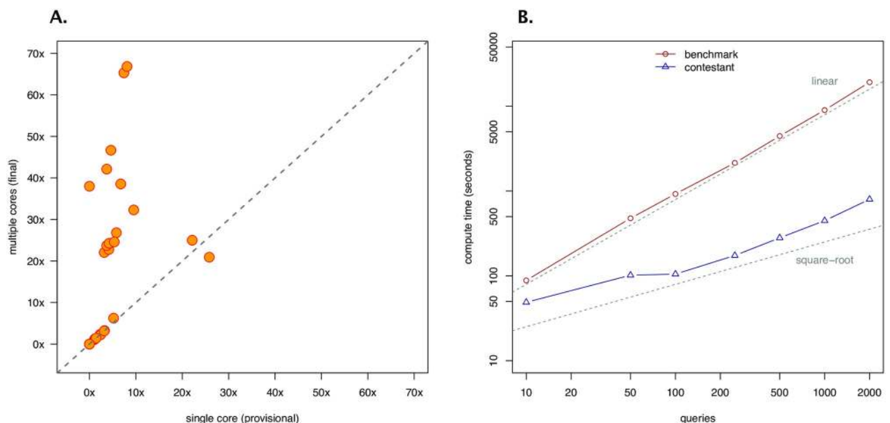
Fig 5. Query Speedup Challenge outcomes. (A): Scatter plot showing the relationship between speedups computed on the participants’ last submission with one single core (x-axis) and those with multiple cores (y-axis); observations lying on the 45 degrees line correspond to participants who did not use multi-threading in their final submission (with small variation around the line due to differences in the set of queries used to compute the speedups); (B): Plot showing differences in the scaling behavior between the benchmark and the top submission (on a log-log scale); for both, the displayed computation times are a median of 10 replicates.
