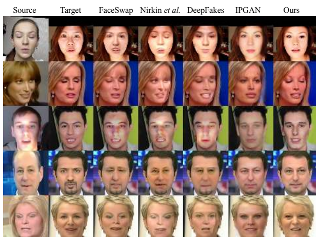
Figure 5: Comparison with FaceSwap [2], Nirkin et al. [31], DeepFakes [1], IPGAN [5] on FaceForensics++ [36] face images. Our results better preserve the face shapes of the source identities, and are also more faithful to the target attributes (e.g. lightings, image resolutions).
