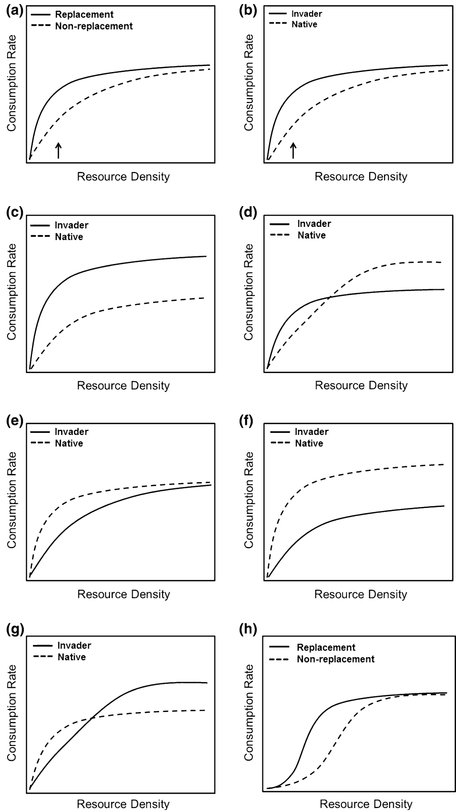
Fig. 3 a–h An illustration of the comparative functional response framework utilising ‘replacement’ study designs (see text for details)
