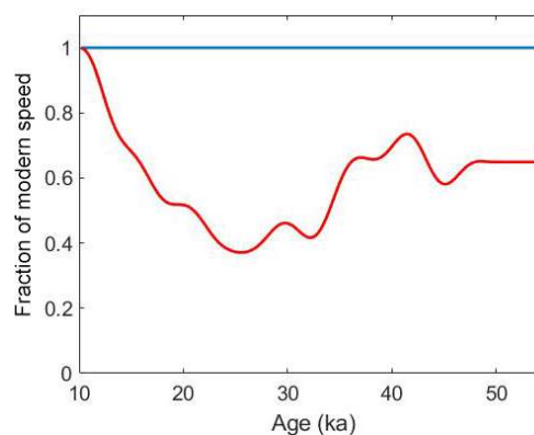
Figure 8. Fraction of modern speed used to reconstruct flowline position and age for the constant speed scenario (blue) and scaled to accumulation history (red).
