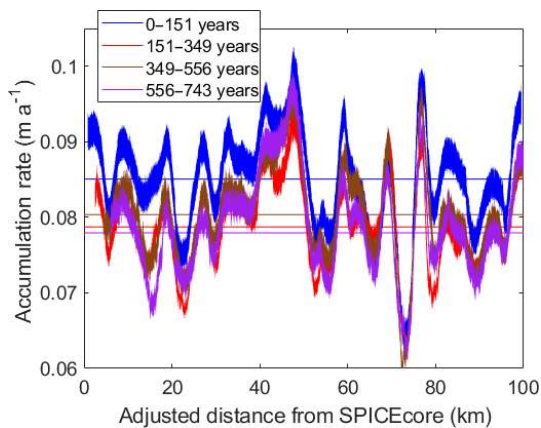
Figure 3. Temporal average accumulation rate for ages between radar layers. Shading indicates uncertainty based on five firn-density profiles. Distance from SPICEcore has been adjusted as in Fig. 2 and described in main text. Horizontal lines indicate spatial average of the accumulation rate using the density profile measured on the firn core at 50 km.
