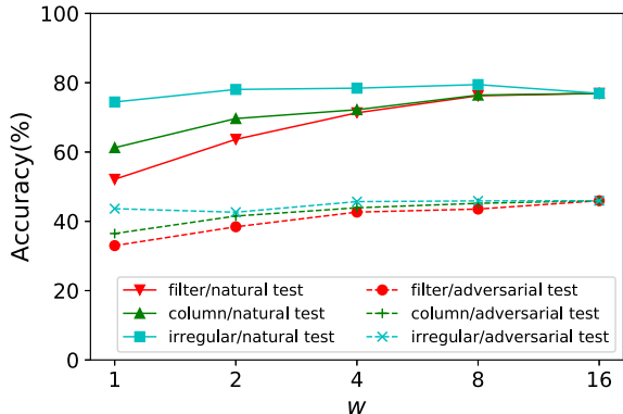
(a) VGG-16
