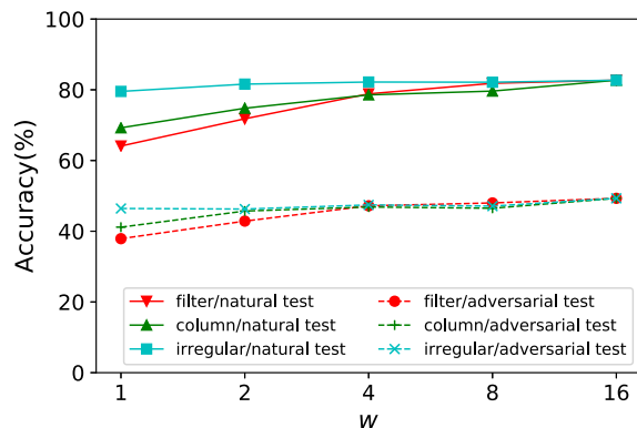
(b) ResNet-18
