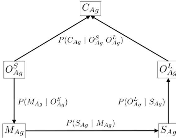
Figure 2. Structure of the communicating agent model, represented with a Bayesian network. Nodes correspond to variables, and arrows represent probability distributions, which illustrate the dependency structure.
