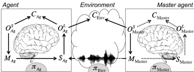
Figure 3. Experimental situation. Several agents populate the environment. On the left, the agent Ag is the focus of interest in our experiments. The other, Master, interacts with it and provides acoustic signals in order to designate an object. Both are instances of the Bayesian communicating agent model. A simulated environment mediates their interaction.
