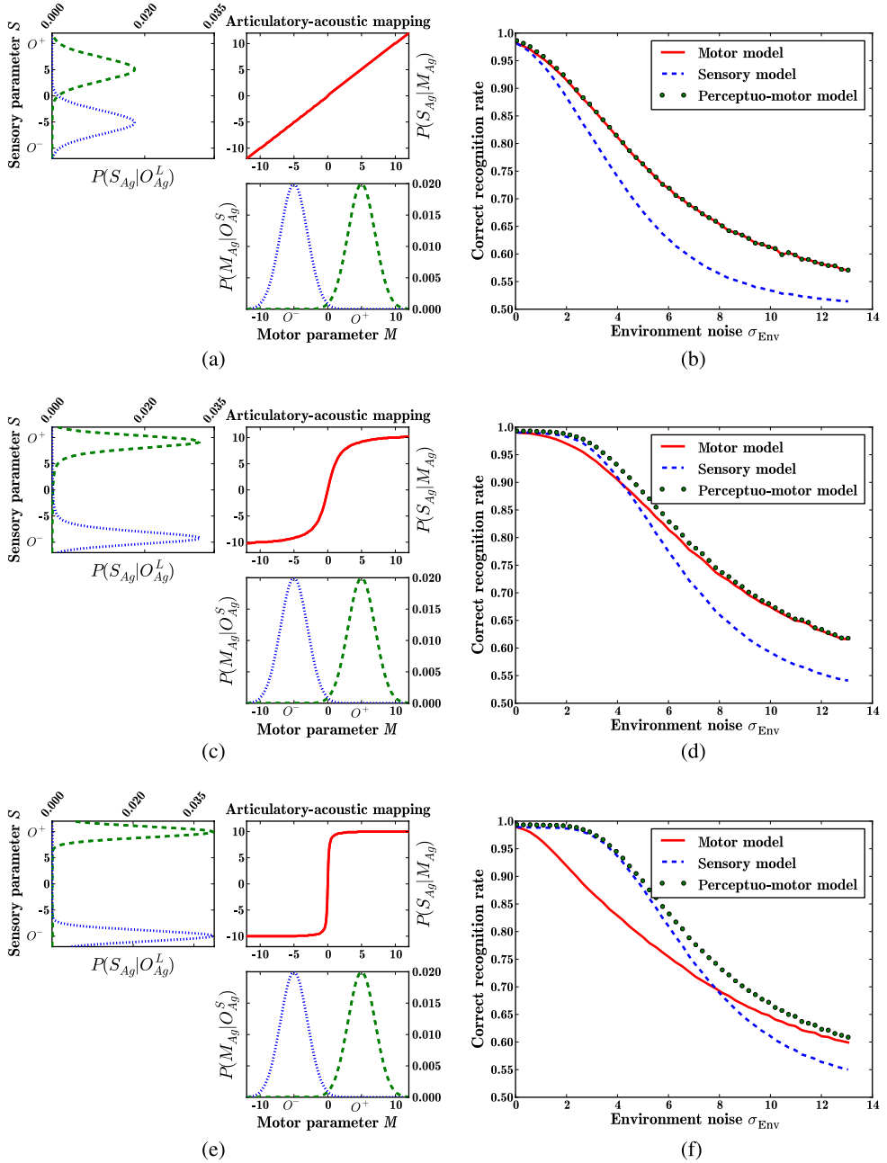
Figure 6. Experimental results for the 1D simulation of communication noise. See text for details. The plots of the left column show the motor prototypes P(M | OS) in the bottom right corner, the articulatory-to-acoustic link P(S | M) (in terms of mean of the sensory variable for a given motor variable) in the top right corner, and the auditory prototypes P(S | OL) in the top left corner. The plots on the right column show the corresponding variations of the correct recognition rate for the different models, when the environment noise \sigma_{Env} varies. Top row: linear case; middle row: nonlinear case; bottom row: strongly nonlinear case.
