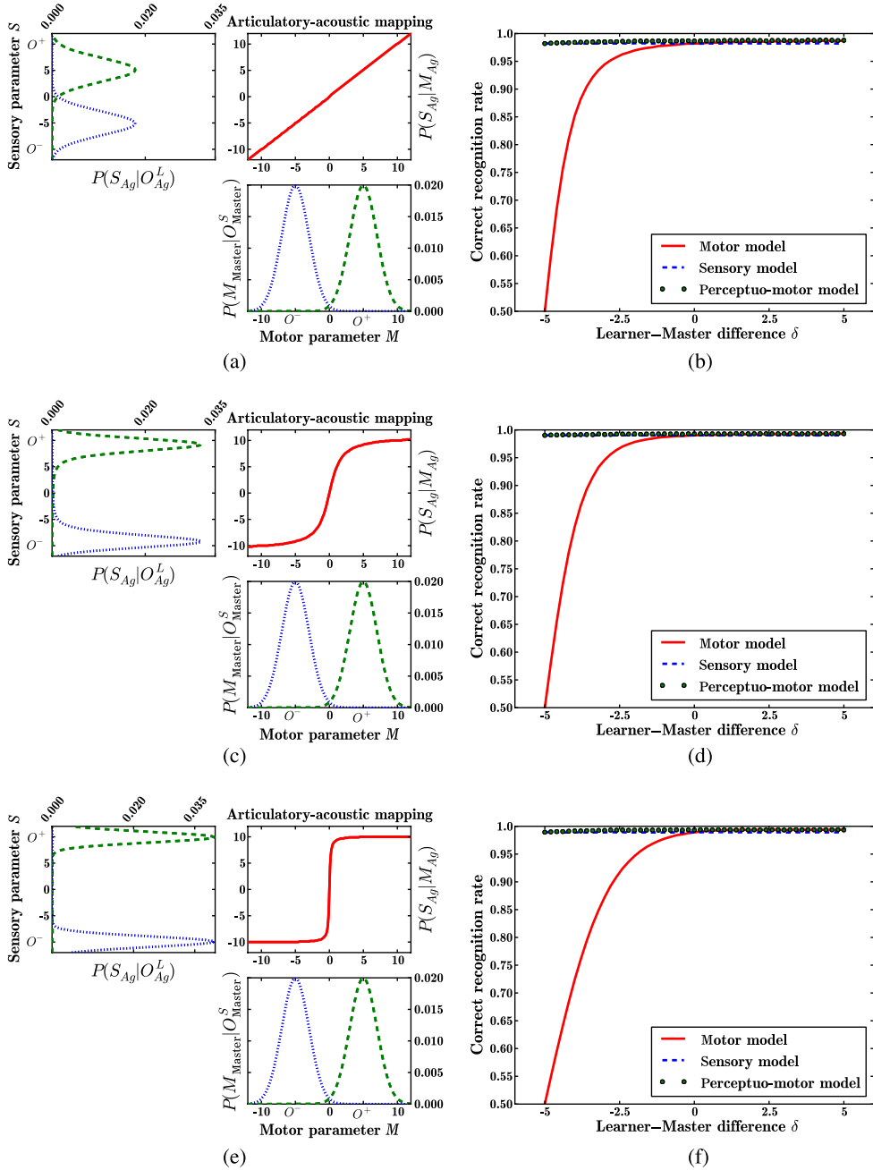
Figure 7. Experimental results for the 1D simulation of variation in motor prototypes between the learner agent Ag and the master agent Master. Same presentation as in Fig. 6. In the right column, the x-axis corresponds to the departure \delta between the Master and Ag agent motor prototypes (0 means equal prototypes in the Master and Ag models).
