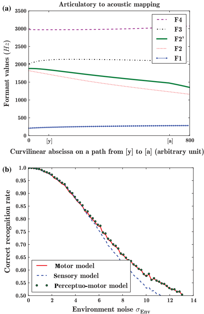
Figure 9. Experimental results for the second 2D simulation: [y]-[a] perception with an almost linear articulatory-to-acoustic transform. (a) Variations of formants (F1, F2, F3, F4) and effective second perceptual formant F2' when mouth opening varies from [y] (on the left) to [a] (on the right). (b) Correct recognition scores for the three models for varying communication noise.
