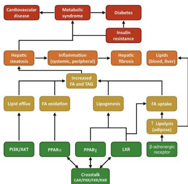
FIGURE 3: Adverse outcome pathway (AOP) network for metabolic disorders mediated by hepatic steatosis. The high level of cross-talk between the different receptors and associated signaling pathways complicates the use of existing high-throughput screening data as predictors of a steatotic outcome. This challenge was overcome by identifying a network topology converging into 4 key events (i.e., lipogenesis, and fatty acid uptake, efflux, and oxidation) that were viewed as critical paths leading to steatosis. Assays measuring these points of convergence integrate the complex interplay of upstream events and translate them into measures that are more directly related to the adverse outcome. FA=fatty acid; TAG=triacylglycerol; PI3K=phosphatidylinositol-3-kinase; AKT=protein kinase B; PPAR=peroxisome proliferator-activated receptor; LXR=liver X receptor; CAR=constitutive androstane receptor; PXR=pregnane X receptor; FXR=farnesoid X receptor; RXR=retinoid X receptor.
