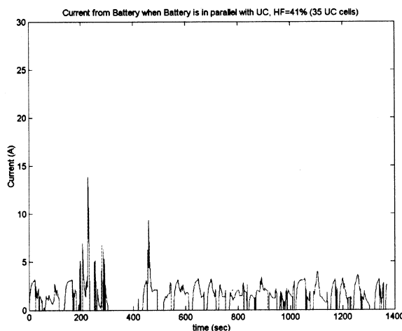
Fig. 3. Current through the battery when assisted by the ultra-capacitor.
