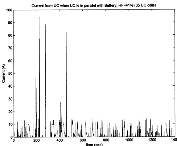
Fig. 4. Current through the ultra-capacitor when it is coupled with the battery.
