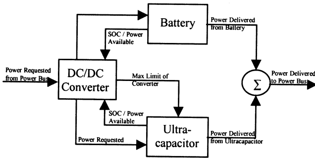
Fig. 1. Block diagram model programmed in Simulink.
