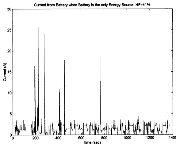
Fig. 2. Current through the battery when the battery is operating as the sole energy source.
