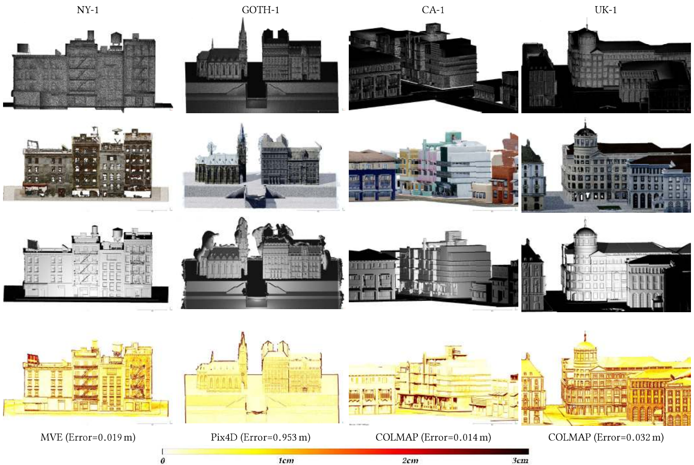
Fig. 13. Quantitative results of large synthetic scene reconstructions. Top Row: input synthetic models with textured Simplex noise, Second Row: reconstruction of the naturally textured models from the SfM pipelines, Third Row: reconstruction of the Simplex noise textured models from the SfM pipelines, Fourth Row: error relative to ground truth point cloud.
