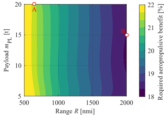
Fig. 6 Aeropropulsive efficiency increase required in order to obtain a 15% increase in PREE, as a function of mission range and payload ( M = 0.55 , \eta_{chain} = 0.9 , CSP = 3 kW/kg, \varphi = 0.2 ). Markers indicate the mission scenarios collected in Tables 3 and 4.
