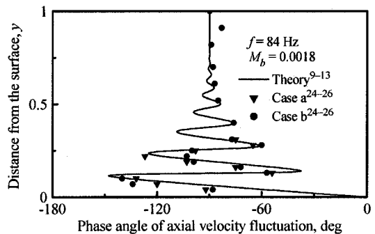
Fig. 3 Comparison of theoretical and experimental phase angles (degrees).
