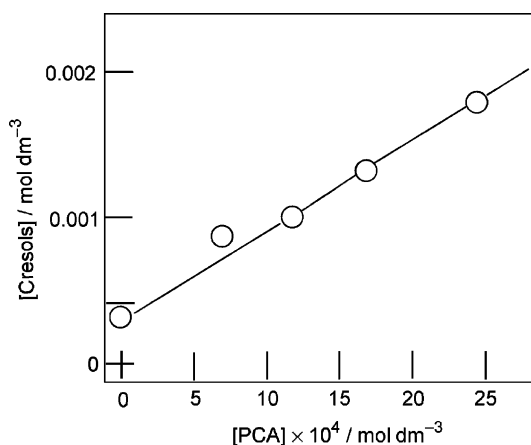
Fig. 4. Concentration of cresol isomers vs. concentration of PCA in the oxidation of toluene ( 0.9 \text{ mol dm}^{-3} ). Conditions: [\text{VO}_3^-] , 2 \times 10^{-4} \text{ mol dm}^{-3} ; [py], 0.08 \text{ mol dm}^{-3} ; [\text{CH}_3\text{CO}_2\text{H}] , 0.67 \text{ mol dm}^{-3} ; ascorbic acid, 0.57 \text{ mmol} ; 30^\circ\text{C} ; 2 h.
