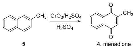
Scheme 3 Commercial synthesis of menadione (BASF). 22
