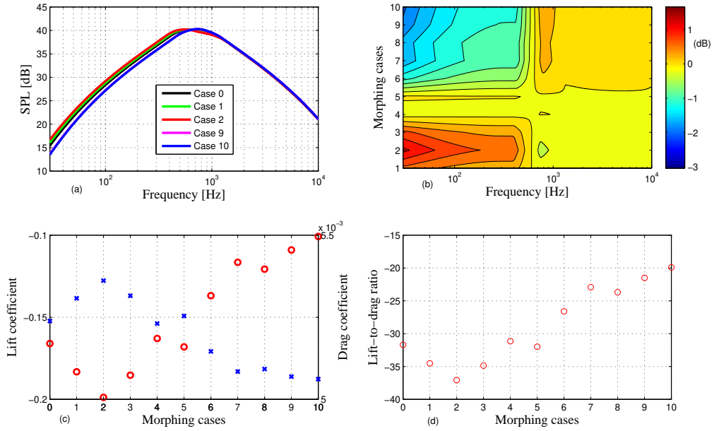
Figure 10. Results of a NACA 63-418 airfoil with a morphing trailing edge (morphing length of b/c = 20\% , deflection angle of \beta = -6^\circ , flow velocity of 50\text{ m/s} and angle of attack of \alpha = 0^\circ ): (a) the SPL of the airfoil; (b) contour plot of noise reduction relative to Case 0; (c) lift and drag coefficients: the cross line represents the drag coefficient and the circle line is the lift coefficient; (d) lift-to-drag ratio.
