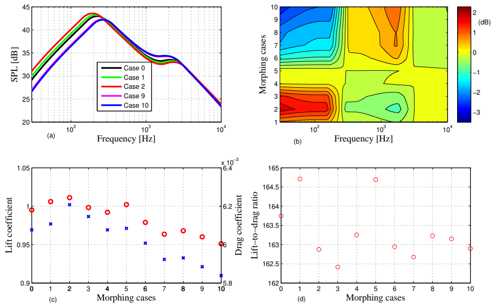
Figure 11. Results of a NACA 63-418 airfoil with a morphing trailing edge (morphing length of b/c = 20\% , deflection angle of \beta = 8^\circ , flow velocity of 50\text{ m/s} and angle of attack of \alpha = 0^\circ ): (a) the SPL of the airfoil; (b) contour plot of noise reduction relative to Case 0; (c) lift and drag coefficients: the cross line represents the drag coefficient and the circle line is the lift coefficient; (d) lift-to-drag ratio.
