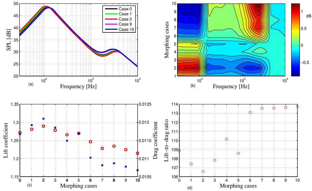
Figure 13. Results of a NACA 63-418 airfoil with a morphing trailing edge (morphing length of b/c = 20\% , deflection angle of \beta = 8^\circ , flow velocity of 50\text{ m/s} and angle of attack of \alpha = 3^\circ ): (a) the SPL of the airfoil; (b) contour plot of noise reduction relative to Case 0; (c) lift and drag coefficients: the cross line represents the drag coefficient and the circle line is the lift coefficient; (d) lift-to-drag ratio.
