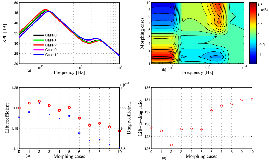
Figure 12. Results of a NACA 63-418 airfoil with a morphing trailing edge (morphing length of b/c = 20\% , deflection angle of \beta = 8^\circ , flow velocity of 50\text{ m/s} and angle of attack of \alpha = 2^\circ ): (a) the SPL of the airfoil; (b) contour plot of noise reduction relative to Case 0; (c) lift and drag coefficients: the cross line represents the drag coefficient and the circle line is the lift coefficient; (d) lift-to-drag ratio.
