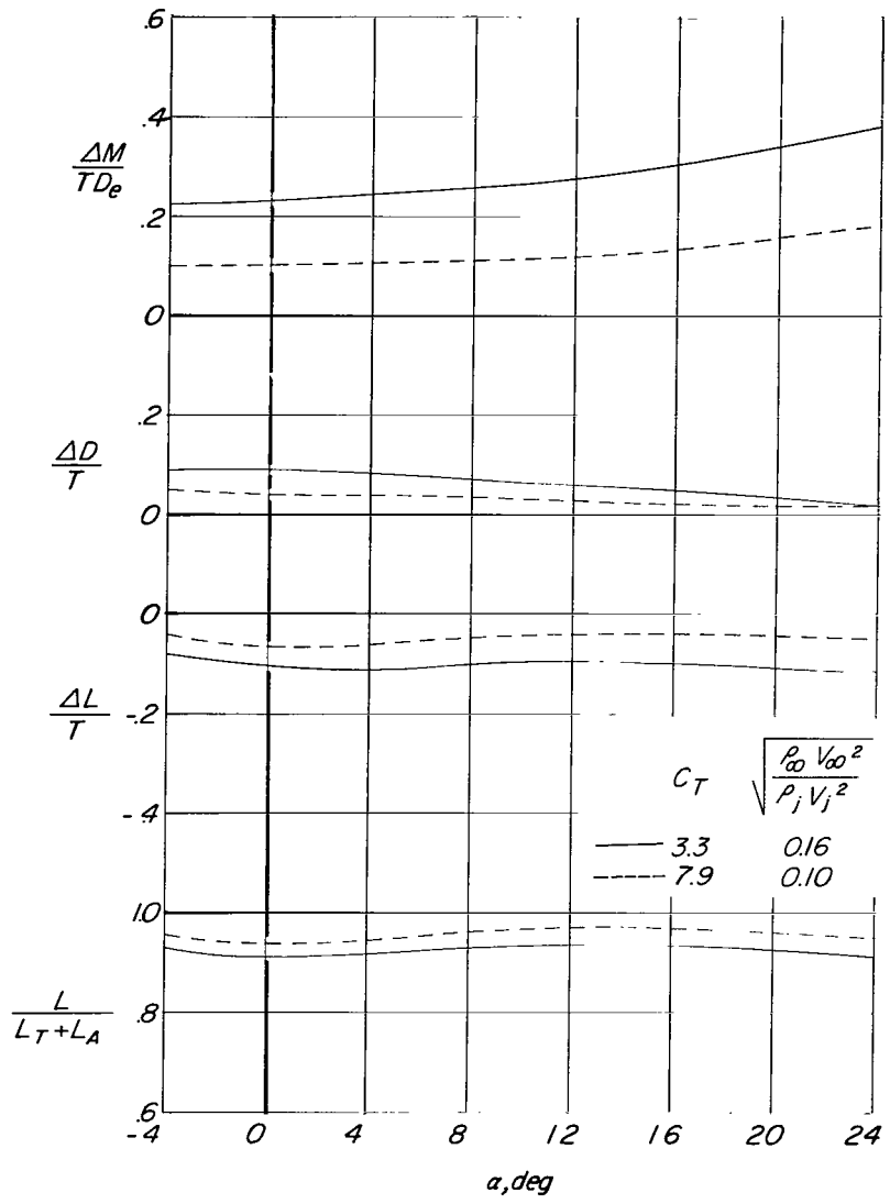
(b) Mid tail position.
