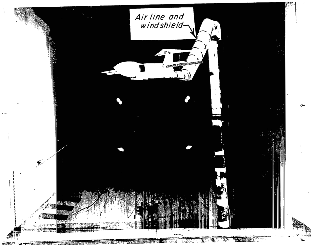
(b) Three-quarter side view of configuration A ( \delta_f = 30^\circ , \delta_s = 35^\circ , fixed forewing) with horizontal tail in high position. L-66-1393
