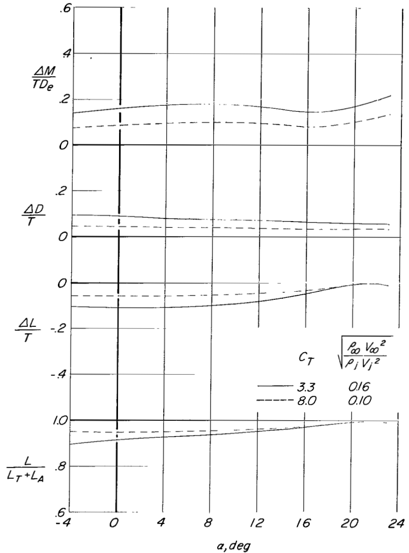
(b) High tail position. Figure 47.- Continued.
