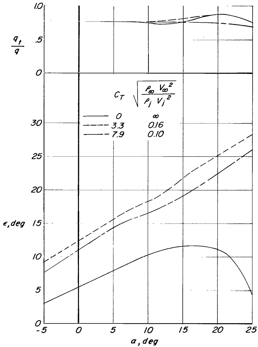
(b) Mid tail position.
