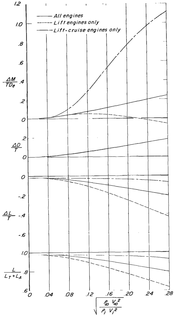
(c) Configuration C ( \delta_f = 0^\circ ).
