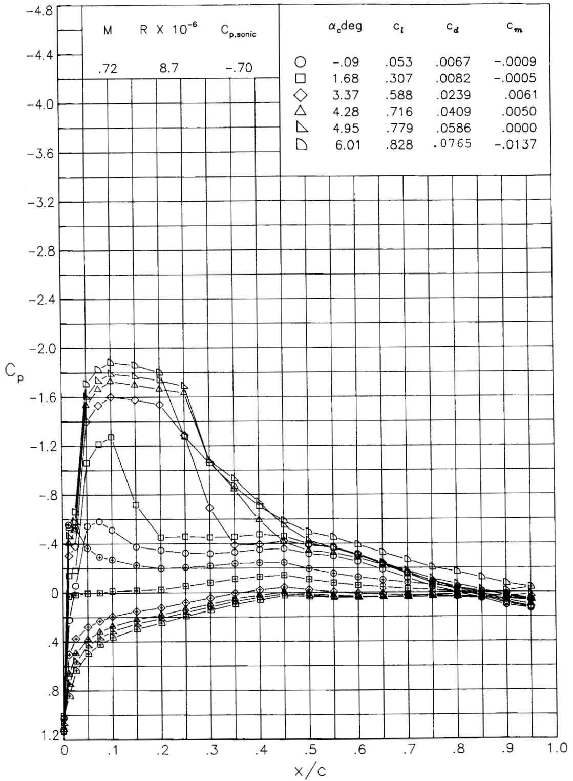
(h) M = 0.72; R = 8.7 \times 10^6 .
