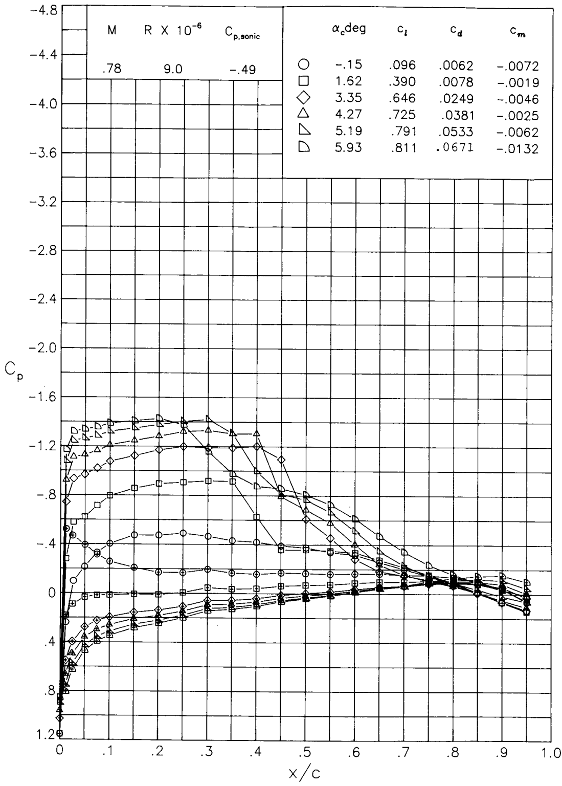
(i) M = 0.78 ; R = 9.0 \times 10^6 .
