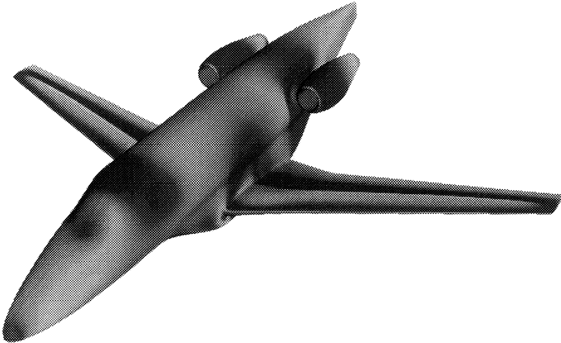
Figure 2: Initial flow solution for wing-body-nacelle geometry. Surface colored by Mach number.
