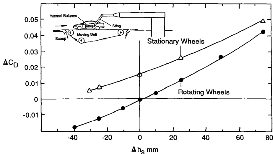
Figure 26 Influence of wheel rotation on drag, as measured for an Opel Calibra over a moving belt in the German-Dutch wind tunnel (DNW); \Delta h_s is the difference in underbody clearance height from the design level.
