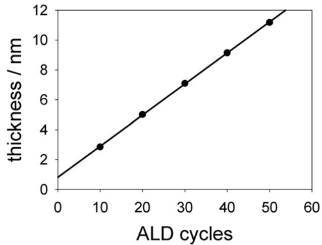
Supplementary Figure 1. Measured thickness of ZnO deposited as a function of ALD cycle. The linear fit indicates self-limiting growth of 0.21 nm / cycle at 150° C.
