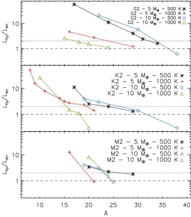
Fig. 4. Ratio between the hydrodynamic ( L_{\text{hy}} ) and energy-limited ( L_{\text{en}} ) escape rates as a function of \Lambda for the modelled planets orbiting the G2 ( top ), K2 ( middle ), and M2 ( bottom ) star. Within each panel, the legend indicates the mass (in M_{\oplus} ) and temperature (in K) of the modelled planets. The dashed line indicates the equality between L_{\text{hy}} and L_{\text{en}} , while the dotted line indicates where the L_{\text{hy}}/L_{\text{en}} ratio is equal to 2.0. The value of \Lambda_{\text{T}} lies between 15 and 35.
