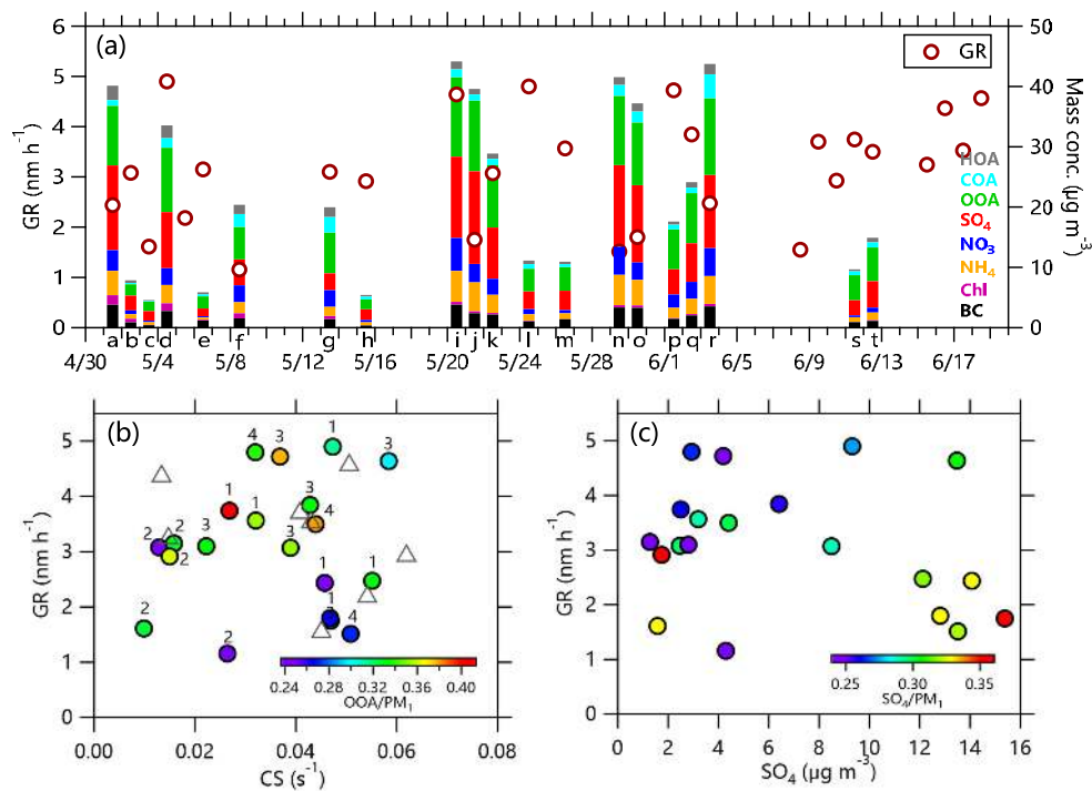
Figure 10. (a) Particle growth rates (GRs) and the corresponding aerosol composition during the growth period, (b) the relationship between GR and CS, color-coded by OOA/PM 1 , and (c) the relationship between GR and sulfate concentration, color-coded by \text{SO}_4 /PM 1 . The numbers over the circles in (b) represent different source regions (Fig. 11) and the triangles represent data without information about composition.
