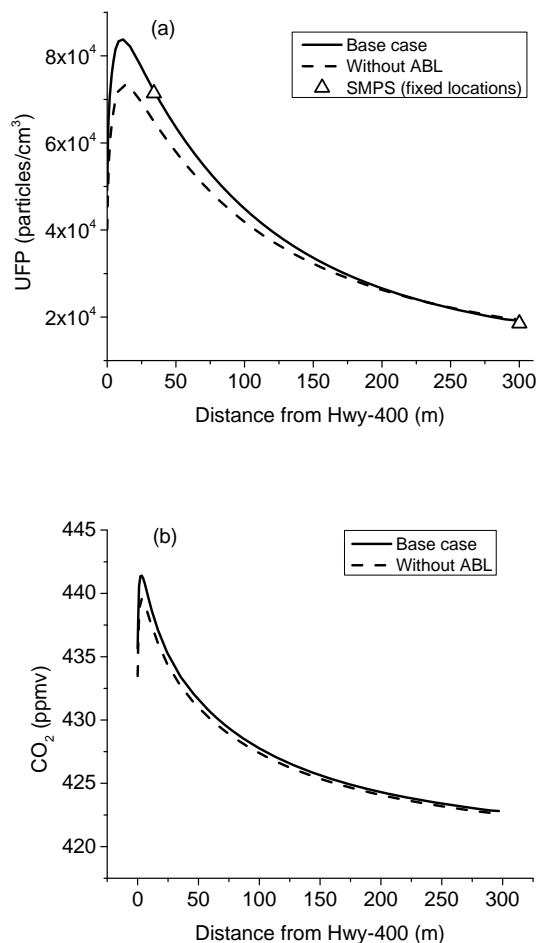
Figure 6. Predicted UFP number (a) and \text{CO}_2 (b) concentrations as a function of distance to the center of Hwy 400.
