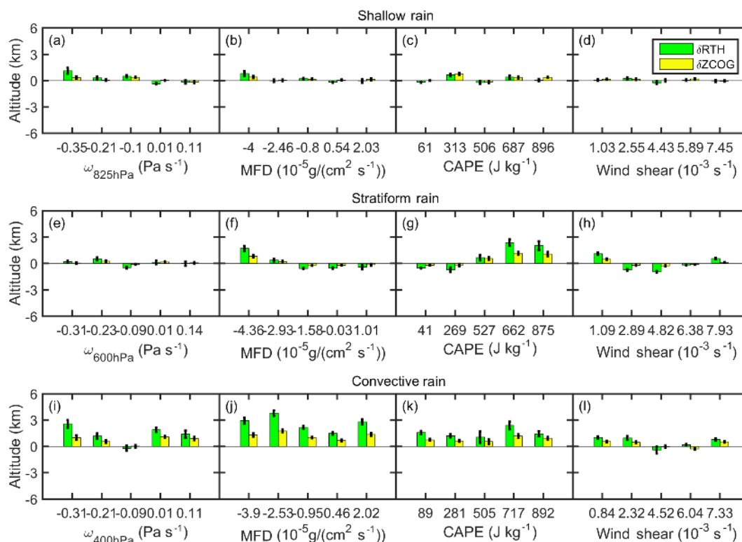
Figure 8. The differences of rain top height ( \Delta RTH) and ZCOG ( \Delta ZCOG) between polluted and clean conditions as a function of different meteorological conditions. (a) \omega at 825 hPa pressure level, (b) MFD, (c) CAPE, and (d) vertical wind shear for shallow regime; (e) \omega at 600 hPa pressure level, (f) MFD, (g) CAPE, and (h) vertical wind shear for the stratiform regime; (i) \omega at 400 hPa, (j) MFD, (k) CAPE, and (l) vertical wind shear for the convective regime. Data are from 2007–2012. Note that negative \omega refers to upward motion. Red and blue colors represent polluted and clean cases, respectively. The vertical error bars represent 1 standard deviation. Each bin in a particular panel is equally spaced and labeled by its average value.
