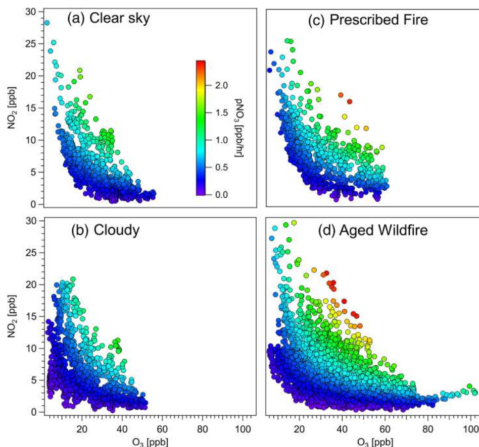
Figure 4. \text{NO}_2/\text{O}_3 plots colored by \text{pNO}_3 . Panel (a) represents typical clear sky conditions, panel (b) represents cloudy and clean conditions, panel (c) represents prescribed-fire (3 hr old) smoke conditions, and panel (d) represents aged (up to several days) wildfire smoke-impacted conditions. Points with both low \text{NO}_2 and low \text{O}_3 during smoke-impacted periods arise from \text{NO}_2 titration of \text{O}_3 and not the inclusion of clear-sky data, which was filtered out as described in section 3.
