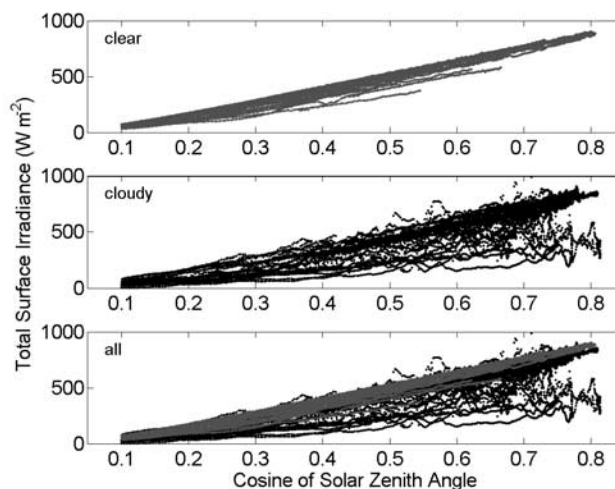
Figure 7. Variation of surface downwelling irradiances with the cosine of the solar zenith angle for (top) cloud-free, (middle) cloudy and (bottom) all data observed in March 2005.
