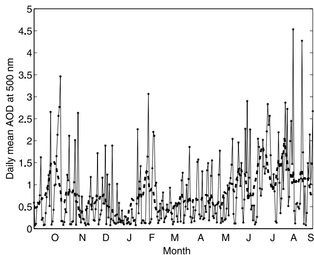
Figure 1. Daily mean aerosol optical depths measured by a Cimel Sun photometer from October 2004 to September 2005 at the Xianghe site. The dashed curve shows the 10-day running averages of the AOD.
