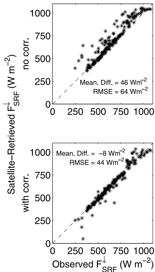
Figure 10. Comparison between satellite-retrieved and surface-observed solar irradiance without and with aerosol corrections using the algorithms of Li et al. [1993] and Masuda et al. [1995].
