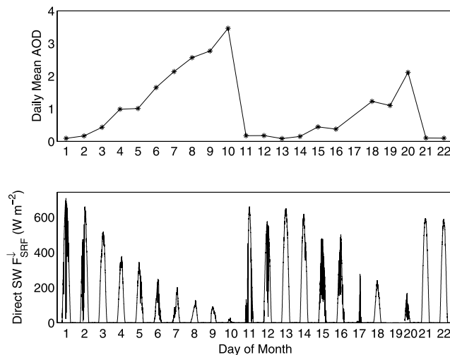
Figure 4. (top) Day-to-day variation of daily mean aerosol optical depths at 500 nm in October 2004 and (bottom) corresponding surface direct solar irradiances.
