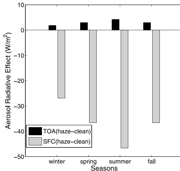
Figure 11. Comparison between the aerosol radiative effects at the top of the atmosphere and at the surface for all matched ground and satellite (CERES) observations.
