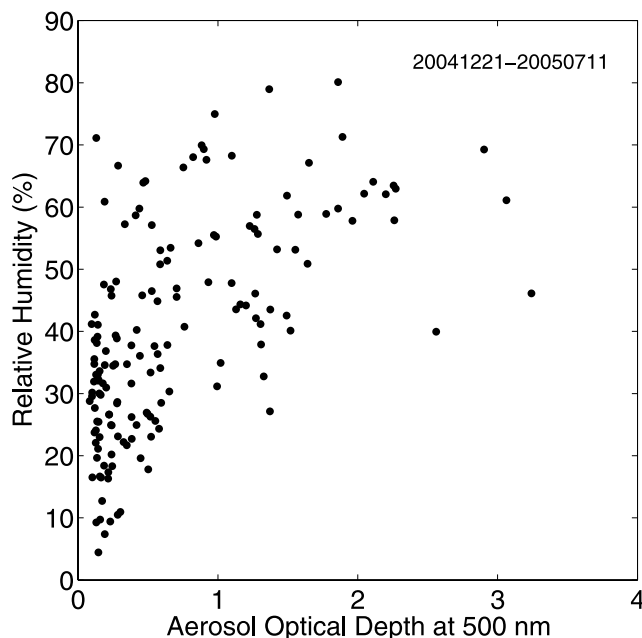
Figure 3. Relationship between the aerosol optical depth and relative humidity for data from 21 December 2004 to 11 July 2005.
