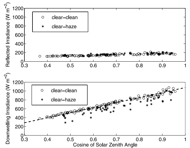
Figure 9. Solar irradiance (top) reflected at the top of the atmosphere (from the CERES SSF product) and (bottom) incoming on the ground (measured) for clear-clean (AOD < 0.2) and clear-hazy conditions (AOD > 0.2).
