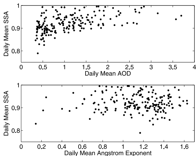
Figure 6. Variations of single scattering albedo with (top) the aerosol optical depth and (bottom) the Angstrom exponent.
