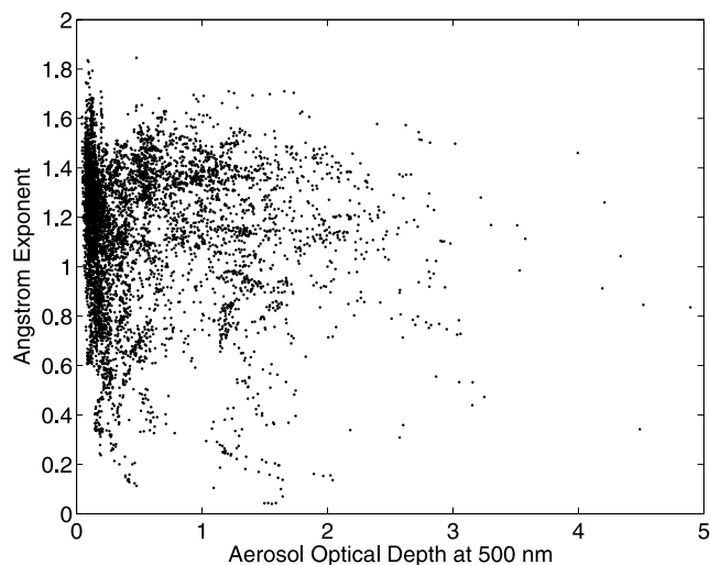
Figure 2. Relationship between the Angstrom exponent and the aerosol optical depth for Cimel data from September 2004 to September 2005.
