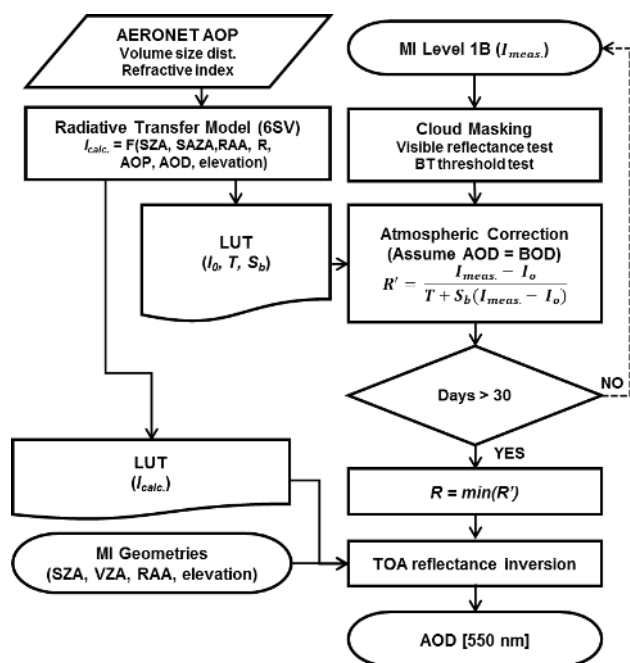
Figure 3. Flowchart of a single-channel algorithm for AOD retrieval, adapted from Kim et al. (2014). I_{\text{meas}} and I_{\text{calc}} represent measured and calculated TOA reflectance, respectively. I_o means atmospheric reflectance including the Rayleigh scattering and aerosol effect, S_b is the hemispheric reflectance, and T is the atmospheric transmittance for the geometry of the sun illumination and satellite viewing. R' shows semi-surface reflectance obtained by correcting the atmospheric effects from the I_{\text{meas}} and the minimum value among the 30-day R' is regarded as the surface reflectance ( R ).
