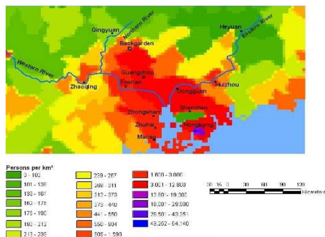
Fig. 1. Map of southeastern China colored by population density (km -2 ). The measurement location (Backgarden) and major cities in the area are labeled. Data source: Socioeconomic data and application center of the Columbia University.
