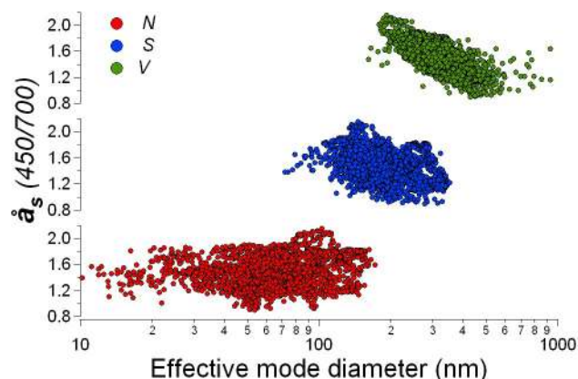
Fig. 18. Ångström exponent ( \hat{a}_s ) vs. the effective mode diameter from mono-modal lognormal fit to measured submicron size distributions of particle number (red dots), surface area (blue dots) and volume (green dots).
