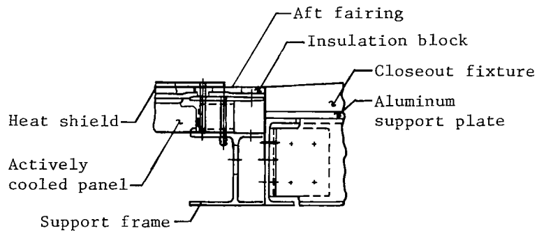
Section C-C aft fairing
