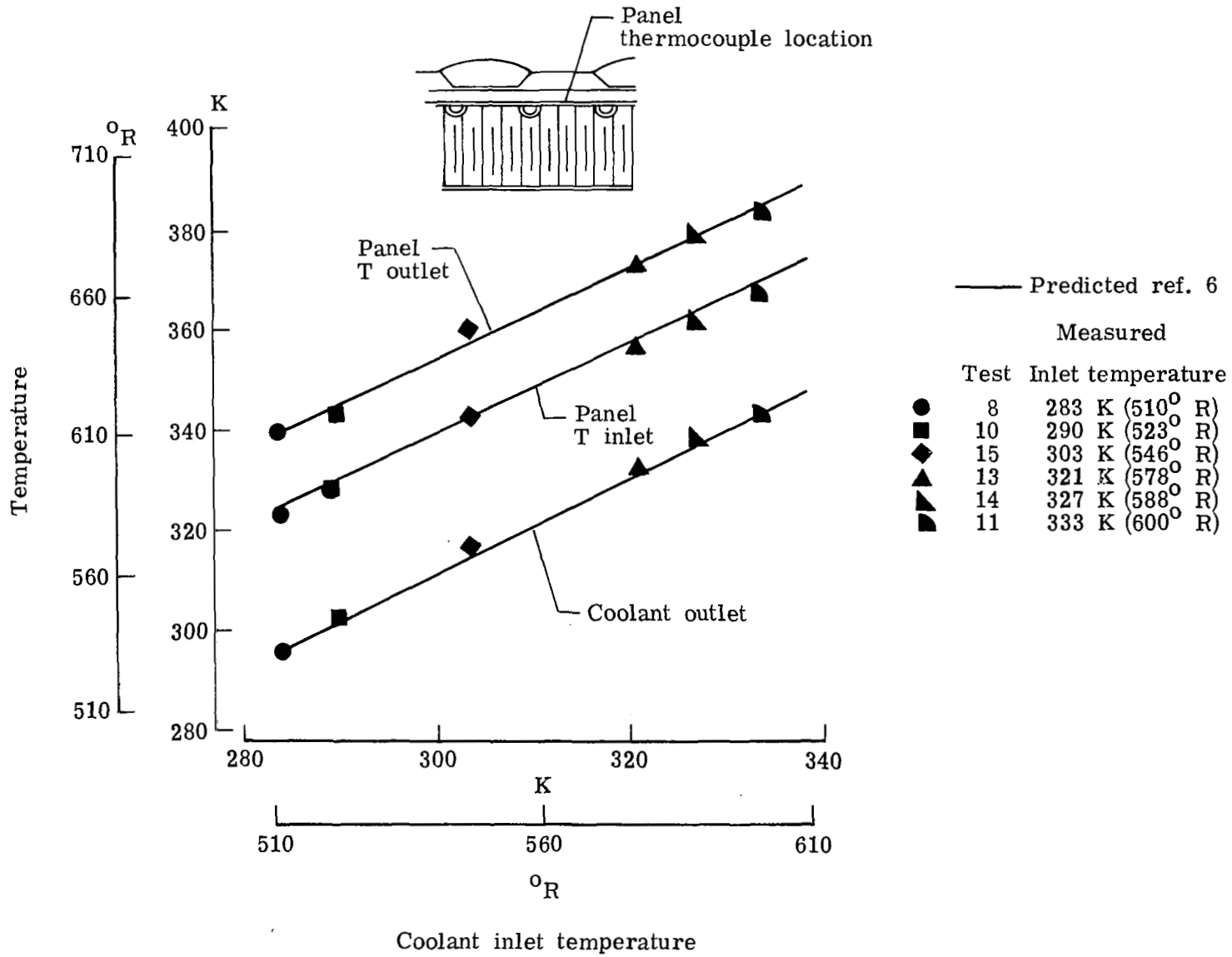
Figure 18.- Comparison of measured and predicted cooled-panel temperatures as function of coolant inlet temperatures.
