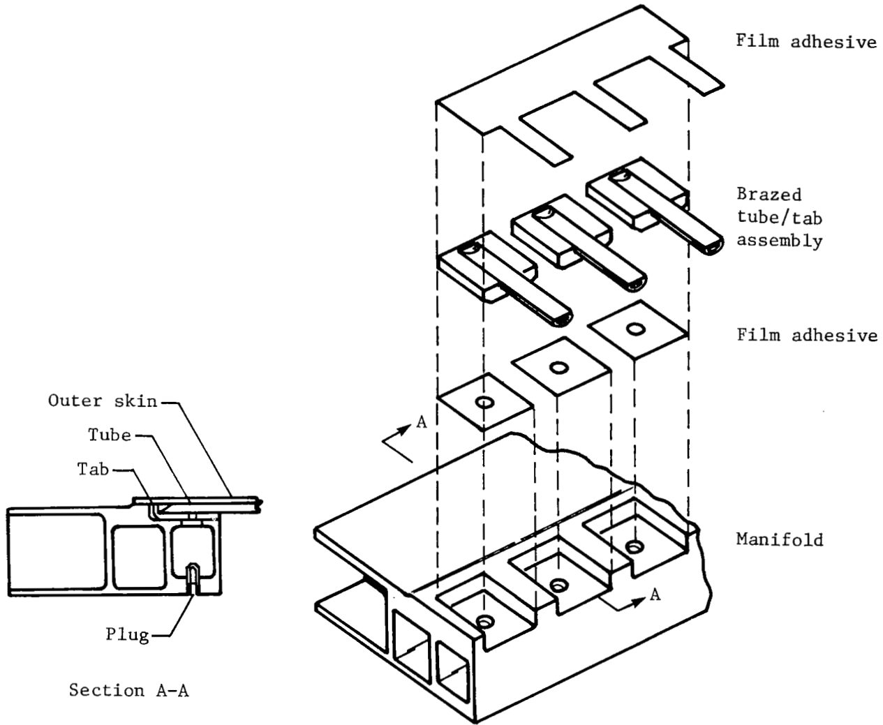
(c) Tube-manifold attachment.
