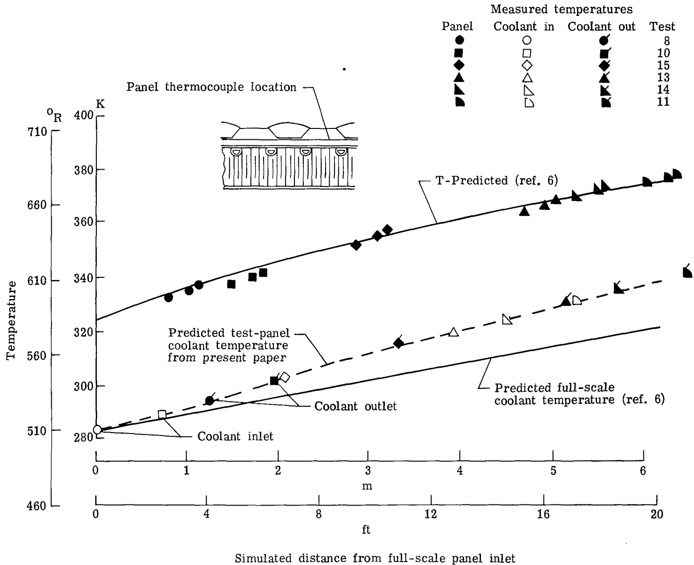
Figure 19.- Comparison of predicted and simulated full-scale (0.61 m (2 ft) by 6.1 m (20 ft)) cooled panel temperatures for RACP.
