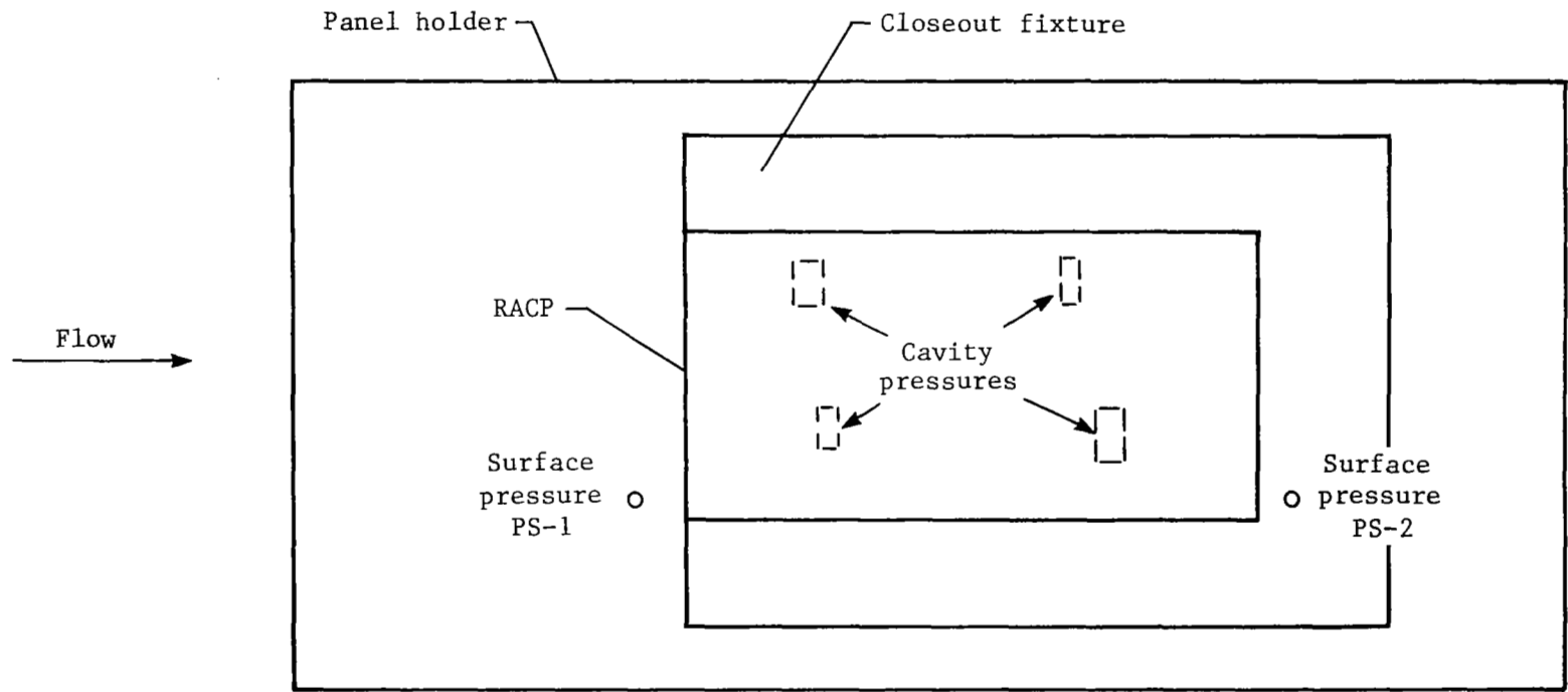
Figure 10.- Instrumentation location for surface and cavity measurements.
