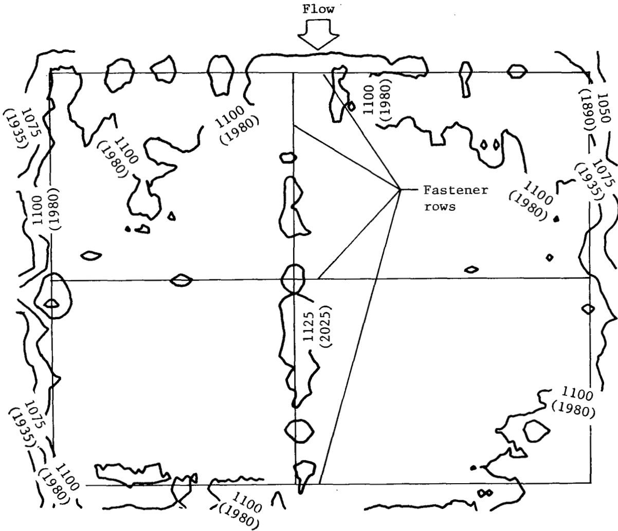
Figure 17.- Heat-shield temperature contours, K (°R), from test 15.
