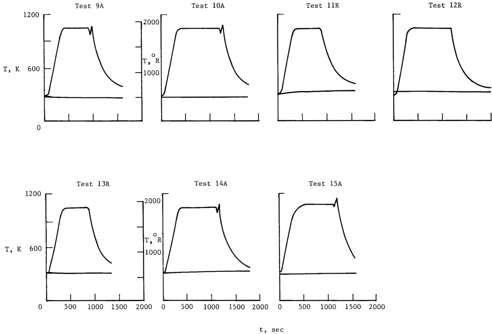
Figure 14.- Concluded.
