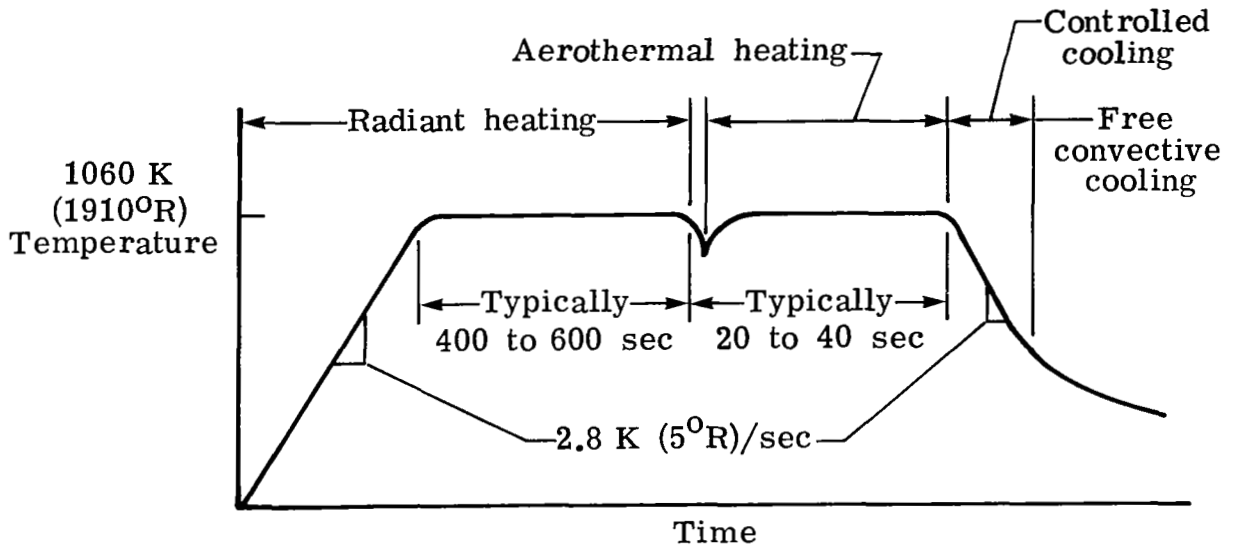
(b) Radiant-preheat aerothermal exposure.
