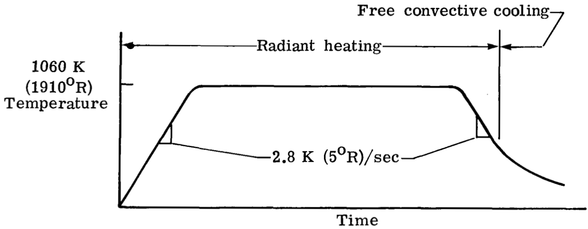
(a) Thermal cycle by radiant heating.
