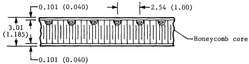
Cooled panel
