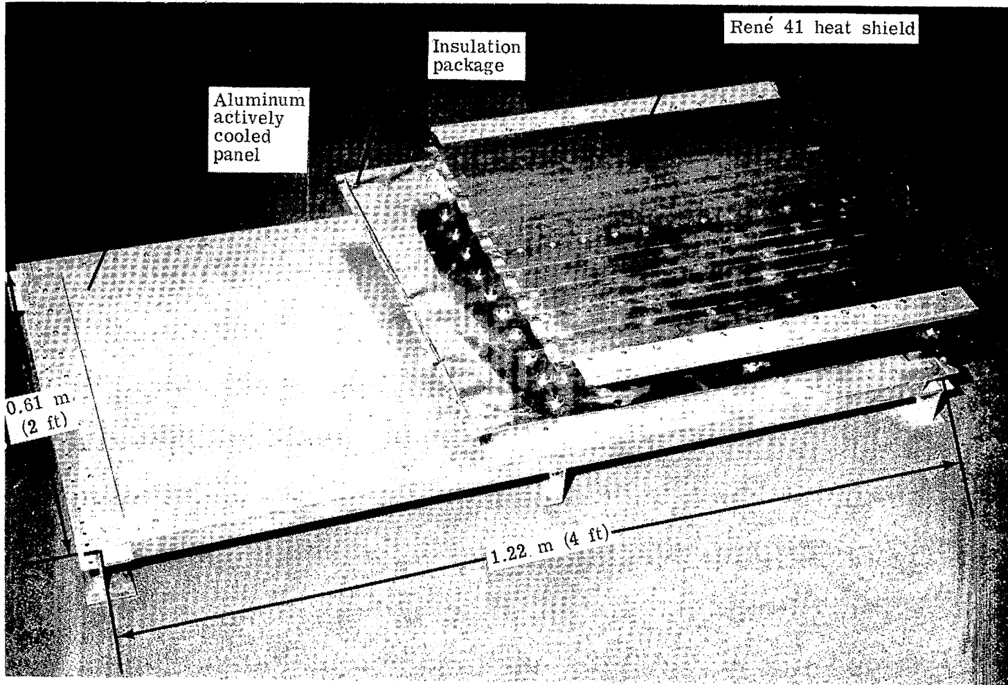
Figure 1.- Radiative and actively cooled test panel.
