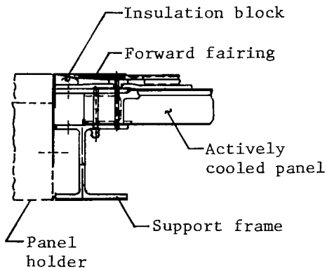
Section A-A forward fairing
