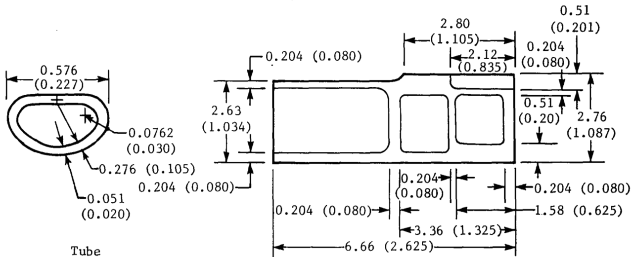
Cooled panel
