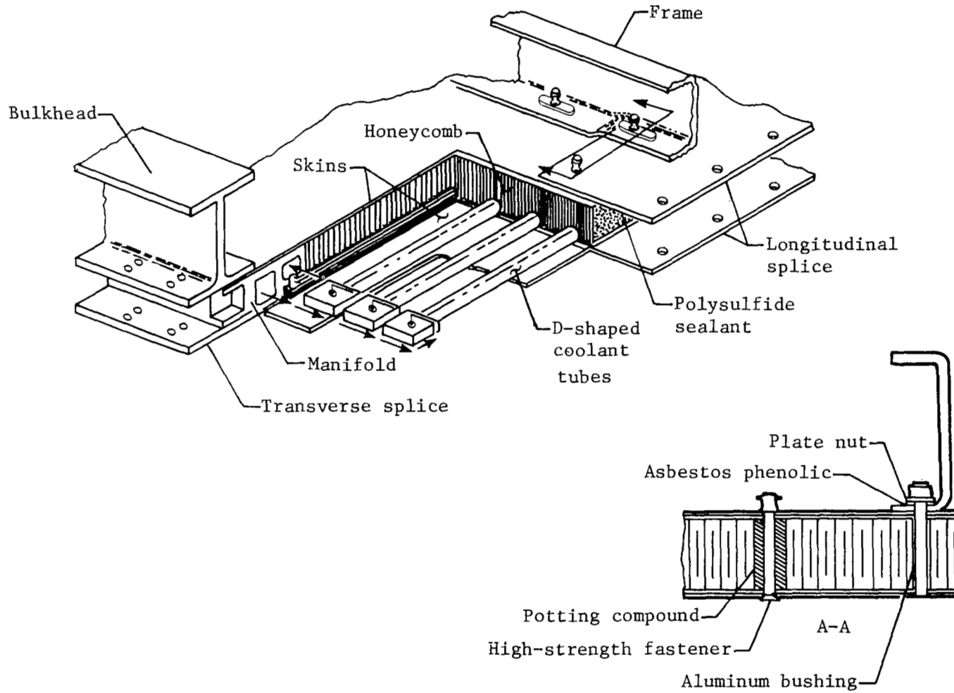
(a) Assembly.
