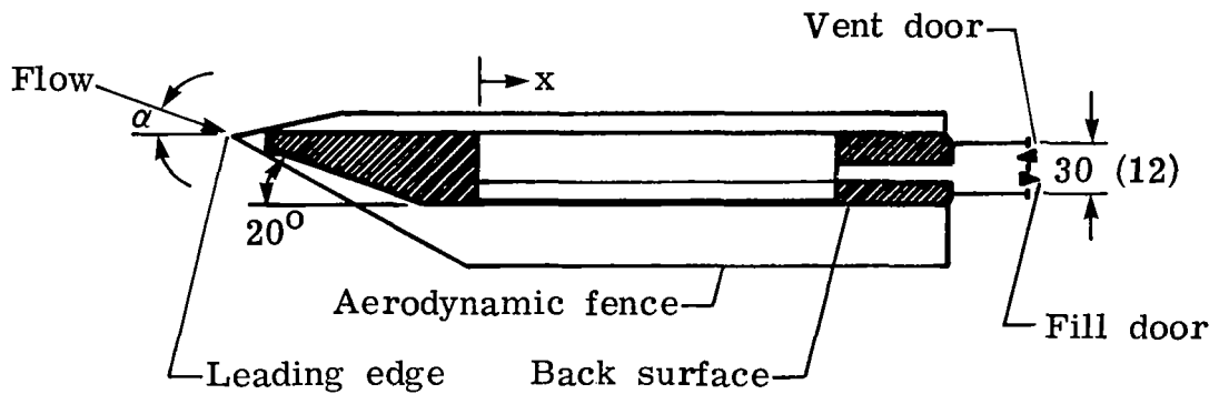
(b) Longitudinal cross section.
