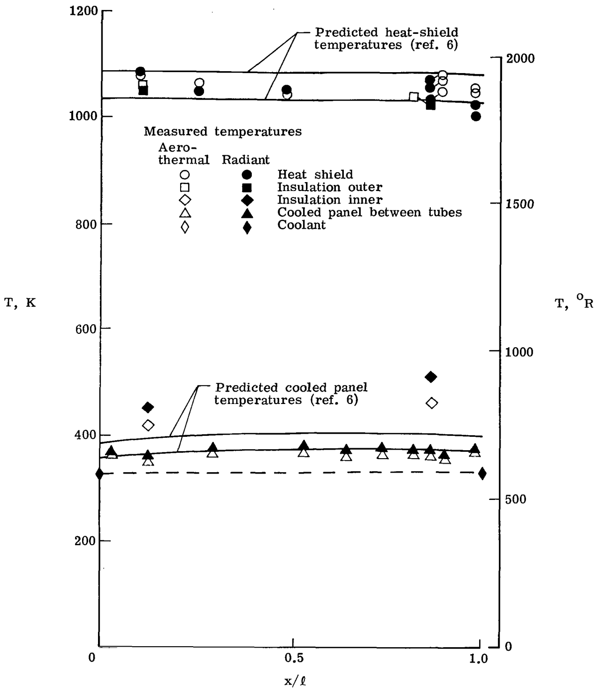
Figure 15.- Comparison of longitudinal temperature distributions from aerothermal and radiant heating for RACP (test 14).
