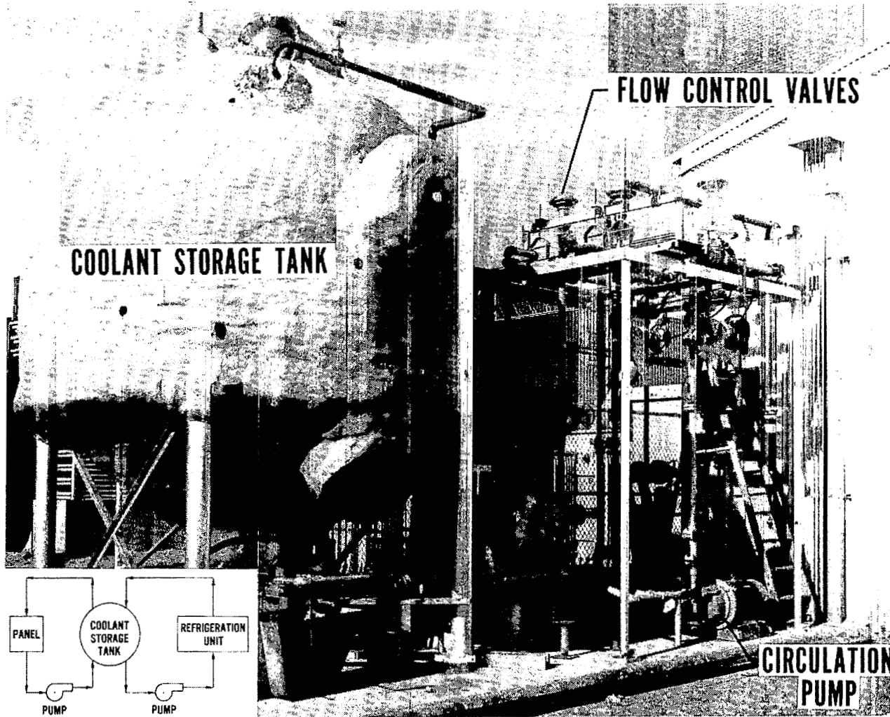
Figure 4.- Test-panel cooling system.
