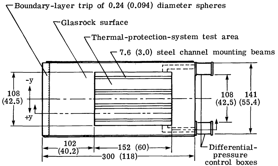
(a) Planview without test panel.
