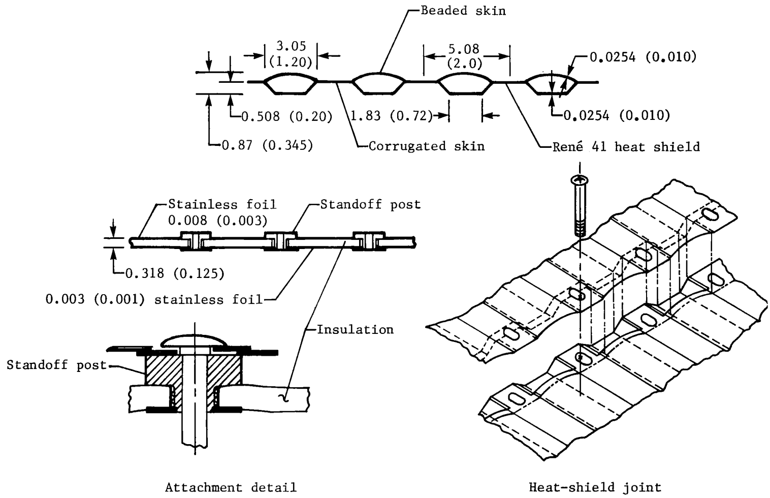
Figure 2.- Heat shield and insulation details. (Dimensions are in cm (in.).)
