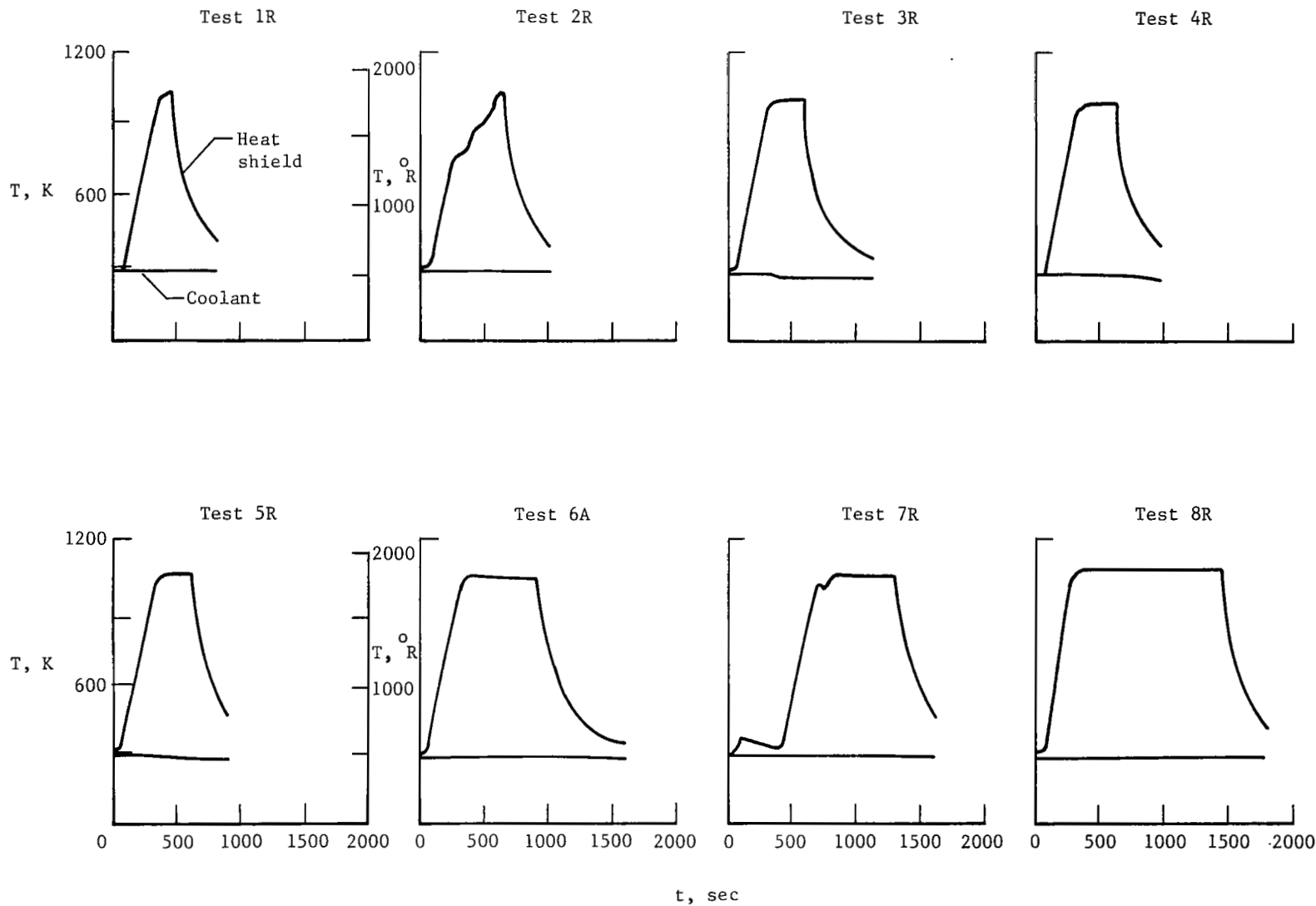
Figure 14.- Heat-shield and coolant inlet temperature histories. (R corresponds to radiant tests; A to aerothermal tests.)
