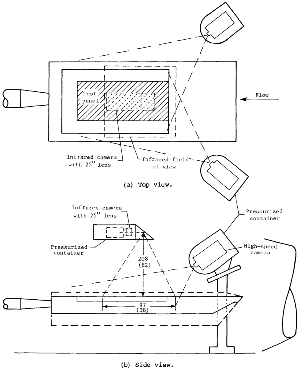
Figure 11.- Camera locations and view angles. (Dimensions are in cm (in.).)
