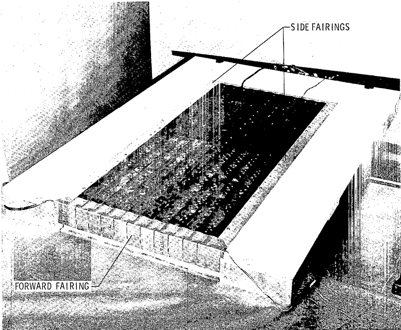
Figure 6.- Test panel mounted in wind-tunnel closeout fixture.
