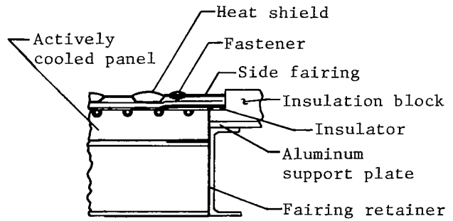
Section B-B side fairing
