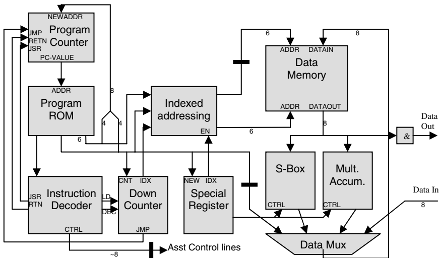
Fig. 5. ASIP Architecture
