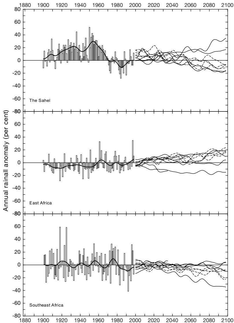
Fig. 13. Observed annual rainfall anomalies for 3 African regions, 1900–98 (see Fig. 3), and model-simulated anomalies for 2000–2099. Model anomalies are for the 10 model simulations derived from the 7 DDC GCM experiments—the 4 HadCM2 simulations are the dashed curves (see Table 1). All anomalies are expressed with respect to either observed or model-simulated 1961–90 average rainfall. The model curves are extracted directly from the GCM experiments and the results are not scaled to the 4 scenarios used in this paper. The smooth curves result from applying a 20 yr Gaussian filter
