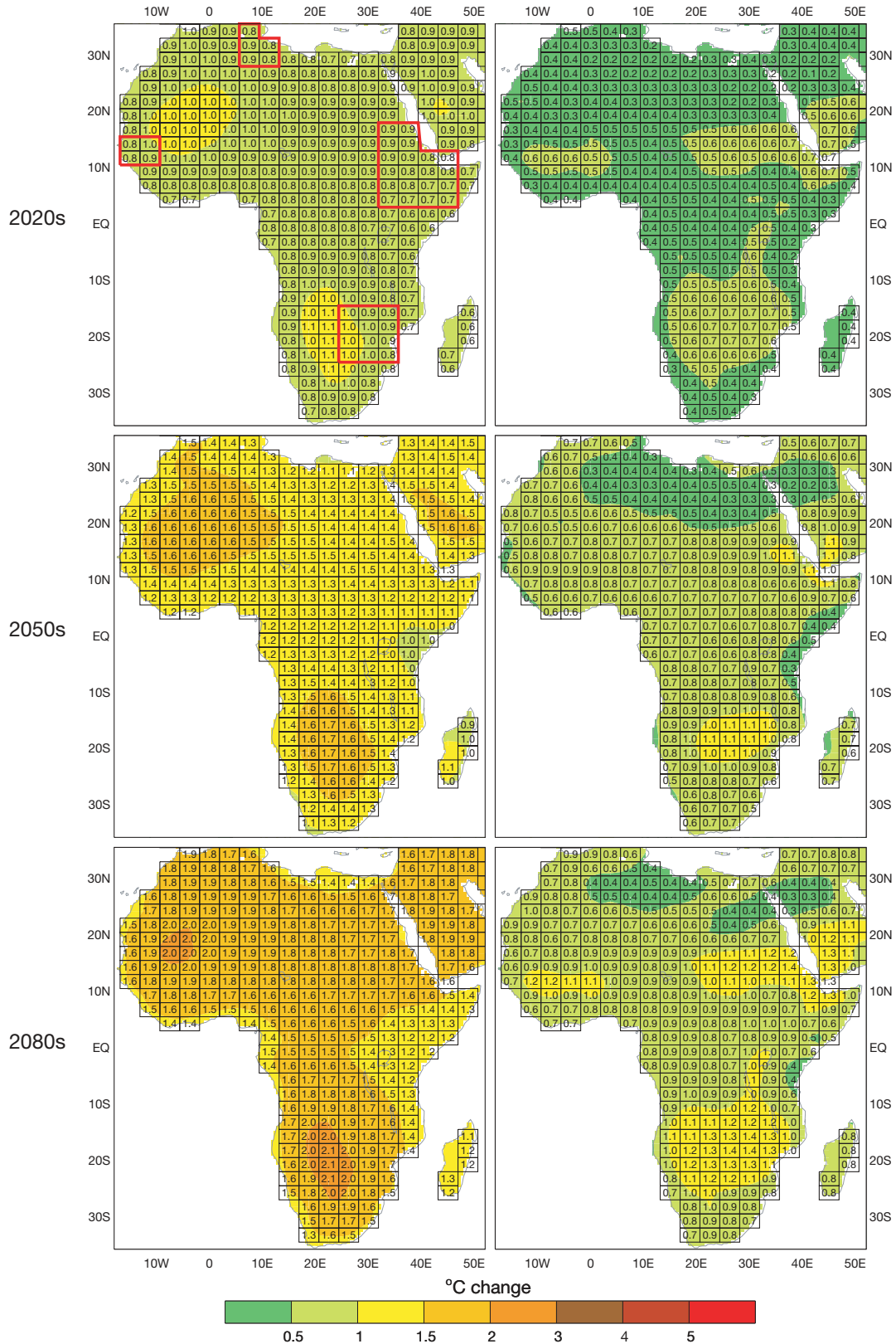
Fig. 6. Left panels: change in mean annual temperature for the 2020s, 2050s and 2080s (with respect to 1961–90) for the B1-low scenario; median of 7 GCM experiments. Right panels: inter-model range in mean annual temperature change. See text for further explanation. Selected domains in the top left panel are the 4 ‘national’ regions used in Fig. 12
