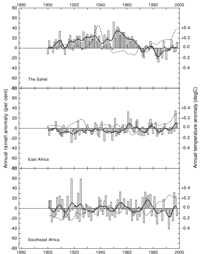
Fig. 3. Annual rainfall (1900–98; histograms and bold line) and mean temperature anomalies (1901–98; dashed line) for 3 African regions, expressed with respect to the 1961–90 average: Sahel, East Africa and southeastern Africa (regional domains marked on Fig. 4). Note: for southeast Africa year is July to June. The smooth curves for rainfall and temperature result from applying a 10 yr Gaussian filter
