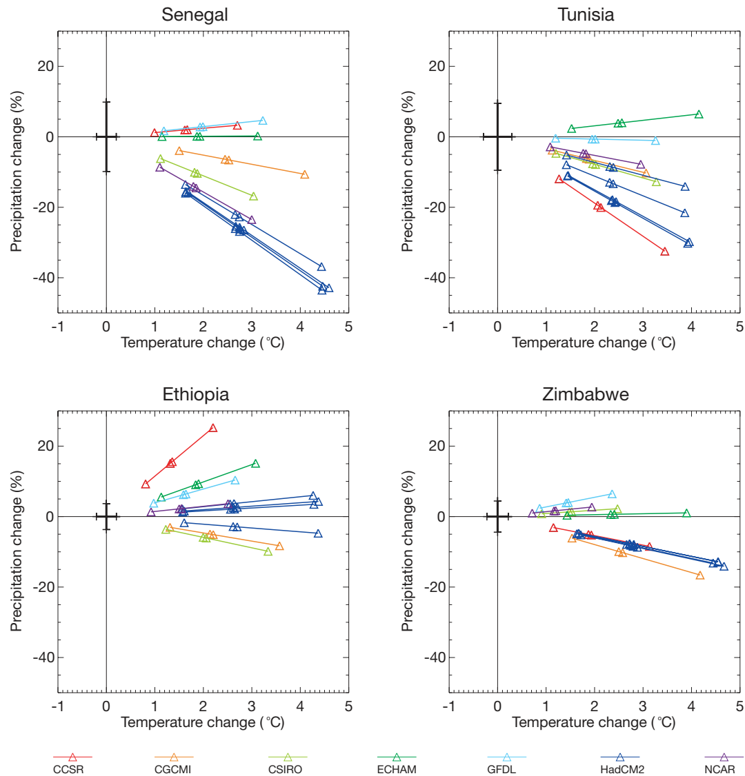
Fig. 12. Change in mean annual temperature and precipitation for the 2050s (with respect to 1961–90) for regions centred on Senegal, Tunisia, Ethiopia and Zimbabwe (see Fig. 6, top left panel, for selected domains). Results from the 7 DDC GCMs are shown, scaled to reflect the 4 climate change scenarios adopted in this study: A2-high, A1-mid, B2-mid and B1-low. Note: the HadCM2 GCM has 4 results reflecting the 4-member ensemble simulations completed with this GCM. The bold lines centred on the origin indicate the 2 standard deviation limits of natural 30 yr time-scale natural climate variability defined by the 1400 yr HadCM2 control simulation
