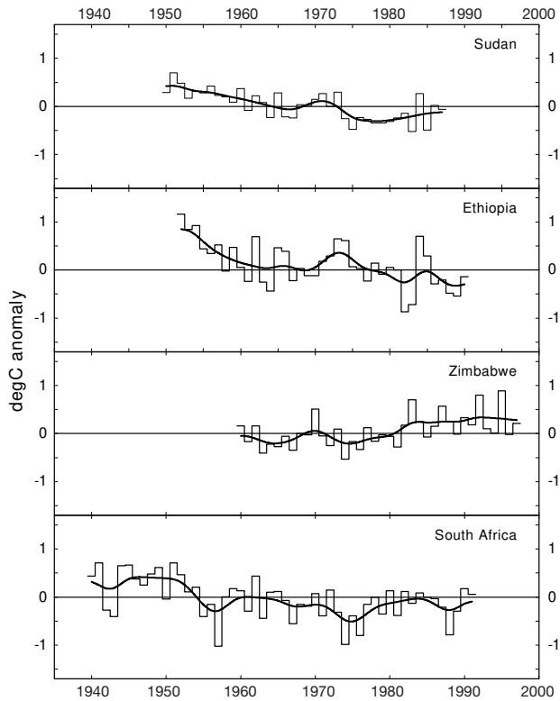
Fig. 2. Mean annual diurnal temperature range ( T_{\max} - T_{\min} ) for a number of African countries: Sudan (data end 1987), Ethiopia (1990), Zimbabwe (1997) and South Africa (1991). The smooth curves result from applying a 10 yr Gaussian filter. Data for Sudan and South Africa are from Jones & Lindesay (1993), while data for Ethiopia and Zimbabwe are unpublished
