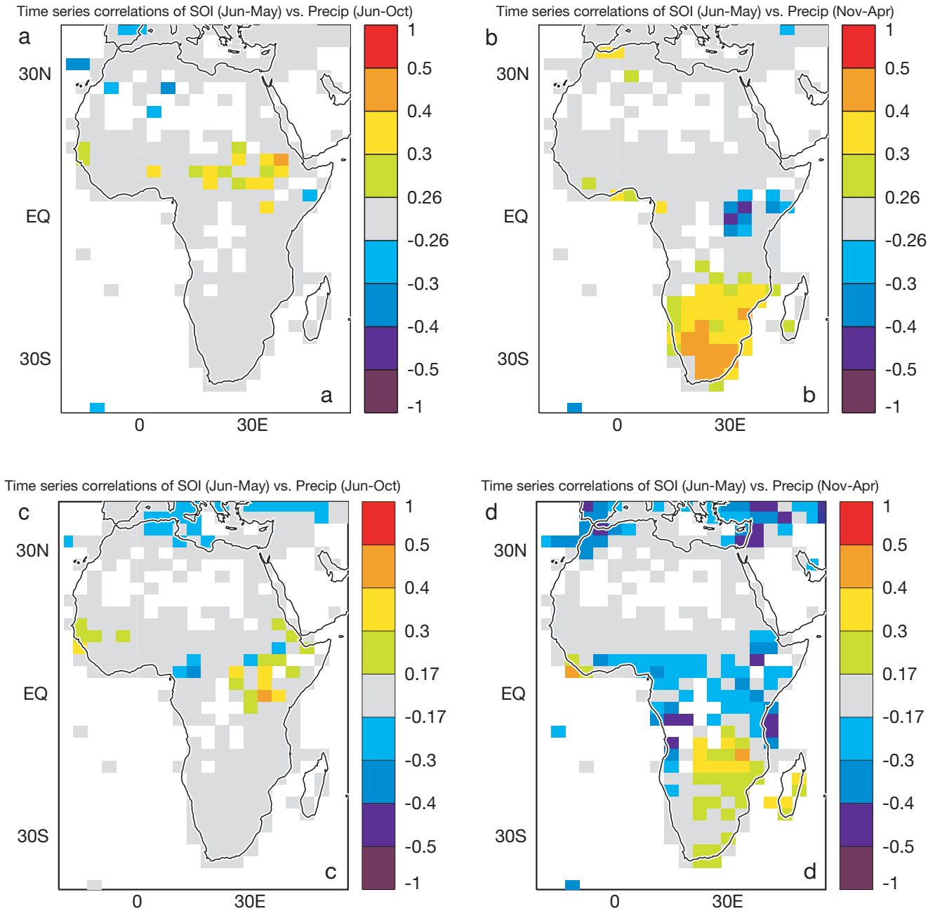
Fig. 5. Correlation between annual (June–May) Southern Oscillation Index (SOI) and seasonal rainfall; (a,c) June–October (Year 0) rainfall; (b,d) November–April (Year 0 to +1) rainfall. (a,b) Observed relationship over the period 1901–98; (c,d) HadCM2 model-simulated relationship over a 240 yr unforced simulation. Correlations are only plotted where they are significant at 95% and in regions where the respective seasonal rainfall is greater than 20 mm and greater than 20% of annual total
