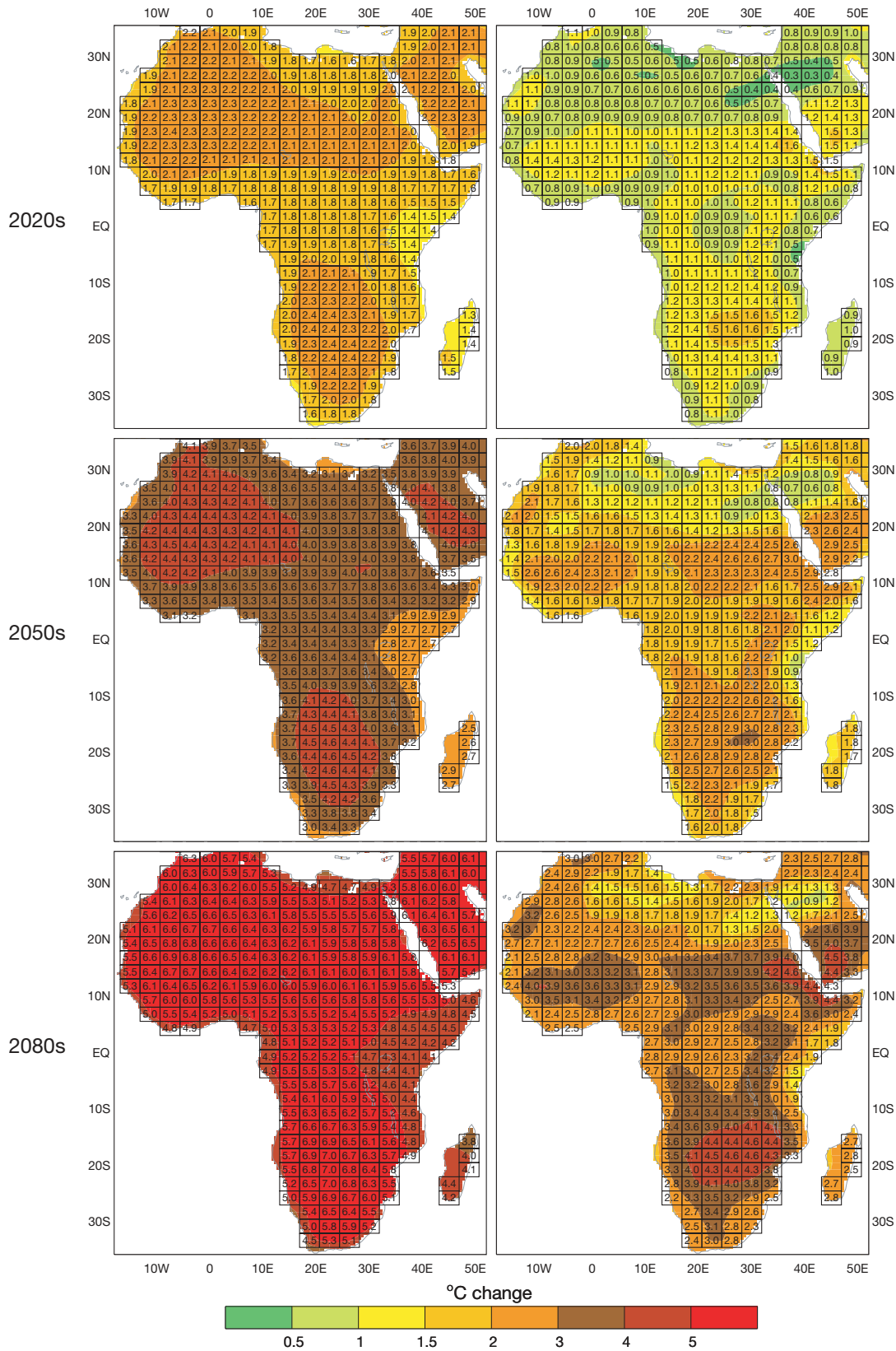
Fig. 7. Left panels: Change in mean annual temperature for the 2020s, 2050s and 2080s (with respect to 1961–90) for the A2-high scenario; median of 7 GCM experiments. Right panels: Inter-model range in mean annual temperature change. See text for further explanation
