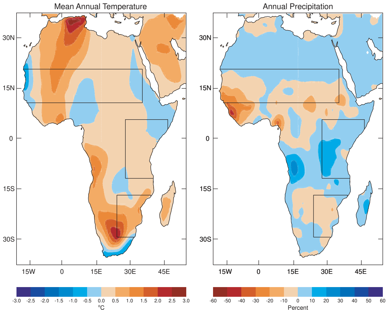
Fig. 4. Mean linear trends in annual temperature (°C century -1 ) and annual rainfall (% century -1 ), calculated over the period 1901–95 from the New et al. (1999, 2000) data set. Data were filtered with a 10-point Gaussian filter before being subject to regression analysis. The 3 regions shown are those depicted in Figs 3 & 13
