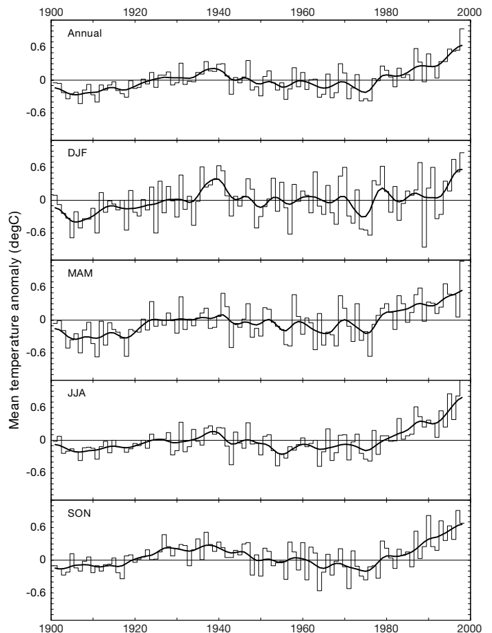
Fig. 1. Mean surface air temperature anomalies for the African continent, 1901–98, expressed with respect to the 1961–90 average; annual and 4 seasons—DJF, MAM, JJA, SON. The smooth curves result from applying a 10 yr Gaussian filter
