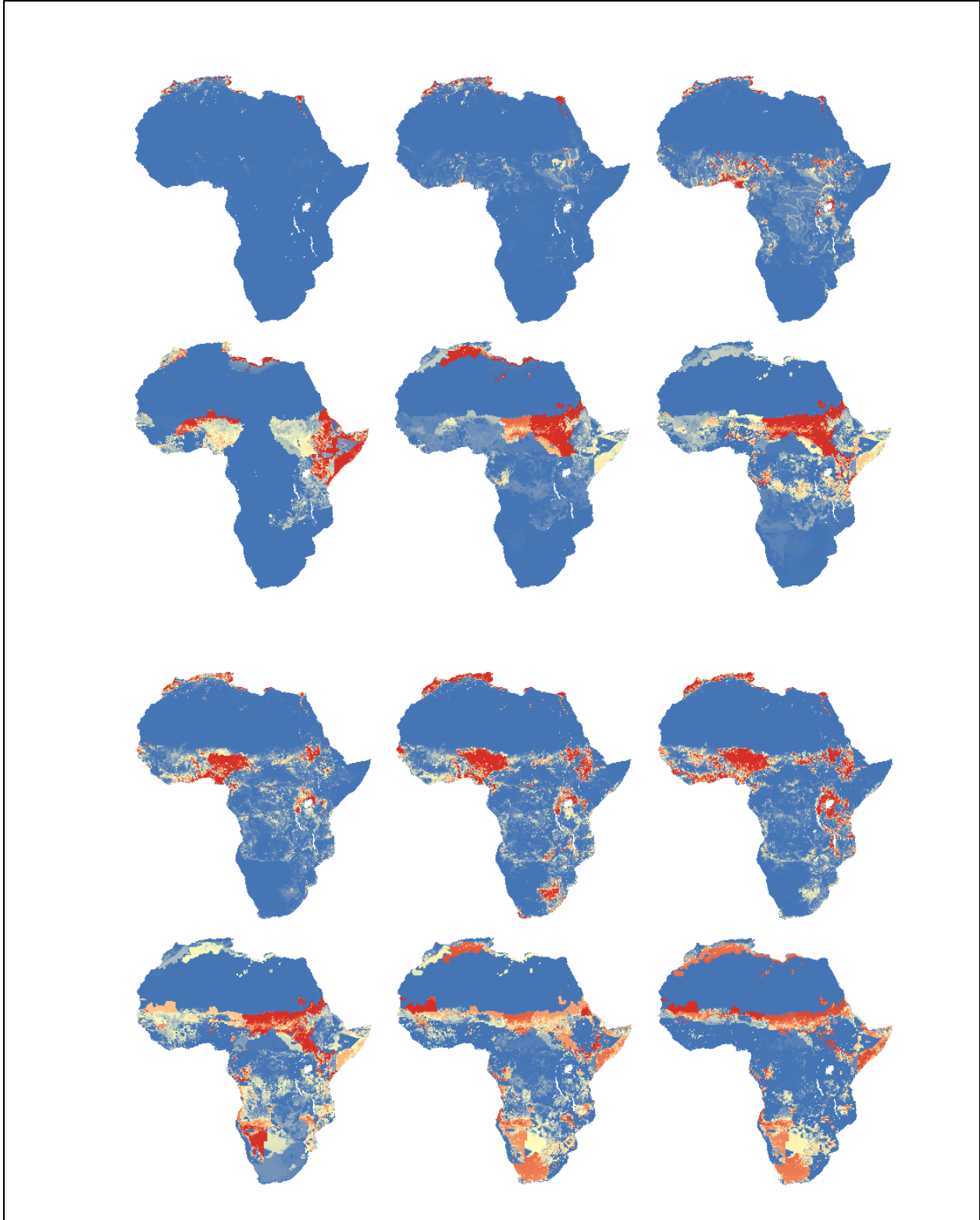
Figure 3 Vegetation change in Africa, 20 kya--present. Adapted from Adams & Faure (66).
