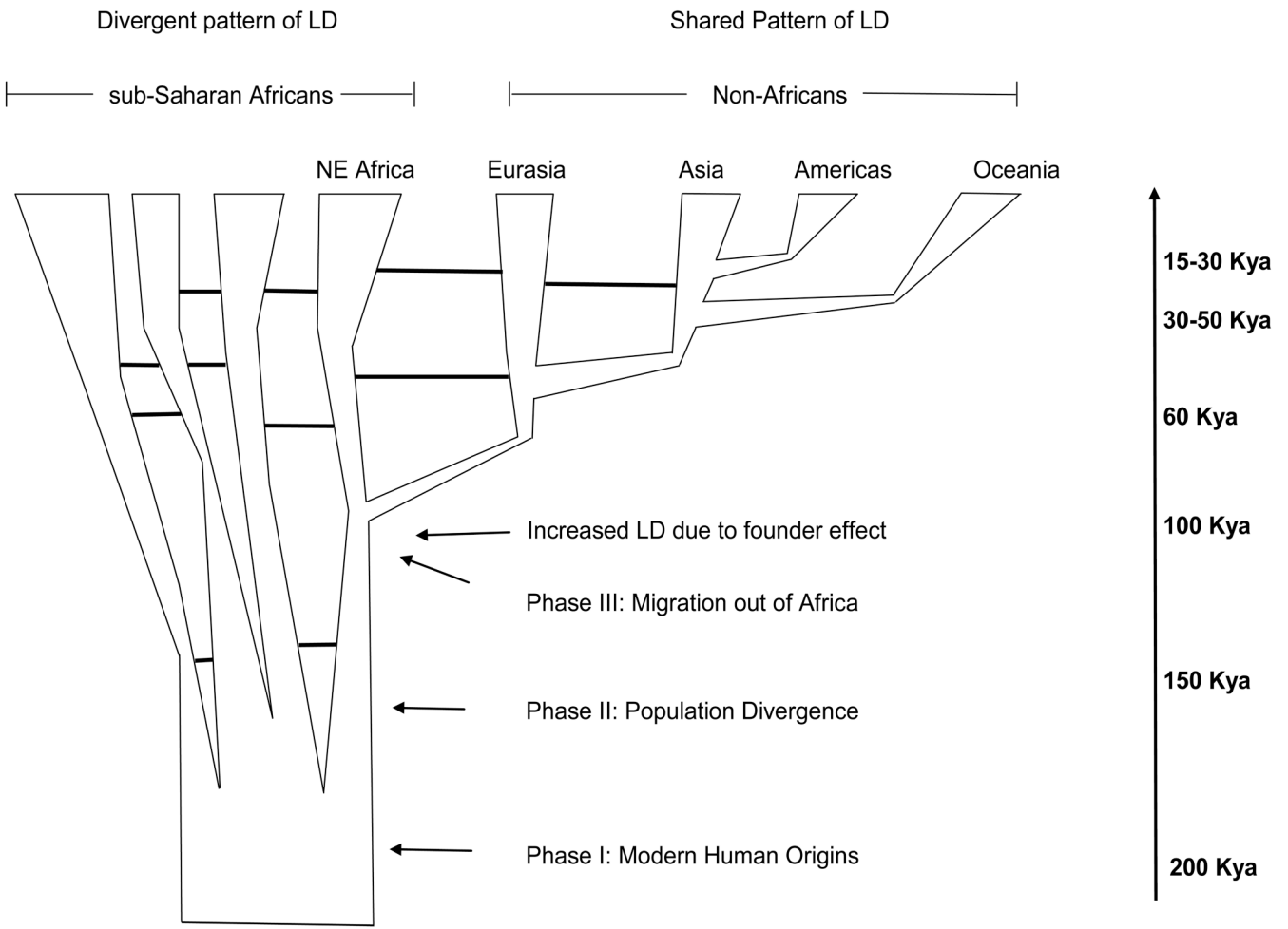
Figure 2. Ancestral Africans have maintained a large and subdivided population structure and have experienced complex patterns of population expansions, contractions, migration, and admixture during their evolutionary history. The bottleneck associated with the founding of non-African populations (~50–100 kya) resulted in lower levels of genetic diversity, an increase in linkage disequilibrium (LD), and more similar patterns of LD. In addition, several recent studies have suggested that a serial founder model of migration occurred in the history of non-Africans in which the geographic expansion of these populations occurred in many small steps, and each migration involved a sampling of variation from the previous population (36,90,109,167). Solid horizontal lines indicate gene flow between populations and the dashed horizontal line indicates recent gene flow from Asia to Australia/Melanesia.
