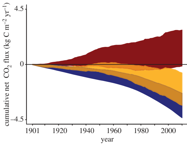
Figure 6. Sensitivity of land carbon storage to atmospheric CO 2 (blue, sink), climate (red, source) and the combined effect of CO 2 and climate (orange, sink) for African humid tropics over the twentieth century for TRENDY land surface models.
