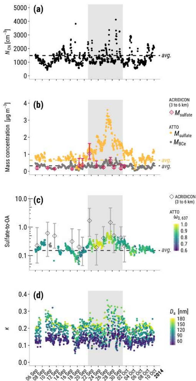
Figure 7. Different aerosol properties measured during the Nya2014 event (gray shaded area), These time series include ATTO hourly averages of (a) aerosol particle number concentration, N_{\text{CN}} , (b) sulfate and \text{BC}_e mass concentration, (c) sulfate-to-OA mass ratio with color-coded aerosol particle single scattering albedo at 637 nm wavelength, and (d) hygroscopicity parameter, \kappa , original time resolution, with color-coded particle activation diameter. Dry season averages are shown as dashed lines. ACRIDICON-CHUVA flight medians and inter-quartile ranges from 3 to 6 km altitude are shown in (b) and (c).
