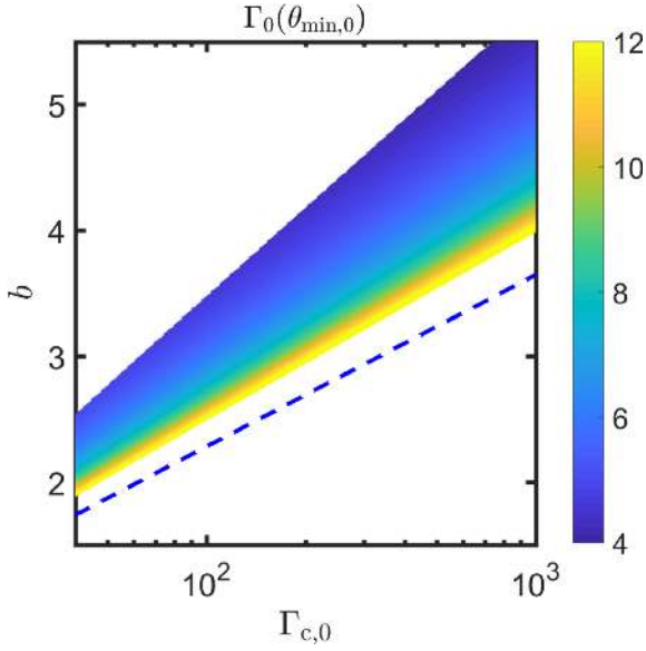
Figure 16. Allowed parameter space provided by the requirements that only one peak is seen in the light curve with t_{\text{pk}} > 7t_{\text{dec}}(\theta_{\text{min},0}) and assuming a = 4.5 , \theta_c = 0.087 , and \theta_{\text{obs}} = 0.47 . Colour represents the value of \Gamma_0(\theta_{\text{min},0}) which in this regime is approximately the initial Lorentz factor of the material dominating the early light curve. A dashed blue line depicts the boundary between cases 1B and 1A (see Fig. 15).
