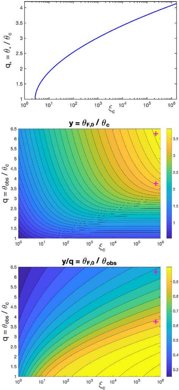
Figure 14. Some key parameters for a Gaussian jet. Top: the angle \theta_* defined by \theta_* \Gamma_0(\theta_*) = 1 (a solution exists for \xi_c \geq e \approx 2.718 ) normalized by \theta_c as a function of \xi_c = (\Gamma_{c,0} \theta_c)^2 (see equation 28). Middle: contour map of the normalized angle y = \theta_{F,0}/\theta_c in the \xi_c - q plane, for PLS G and p = 2.2 (see equation 29); contours are at intervals of 0.1 from y = 0.5 to 3.8, while the two magenta plus symbols in the last two panes are for the two lightcurves shown in Fig. 13. Bottom: a similar contour map of y/q = \theta_{F,0}/\theta_{obs} with contours at y/q = 0.25:0.05:0.95, 0.99, 0.999, 0.9999, \text{ and } 0.99999 .
