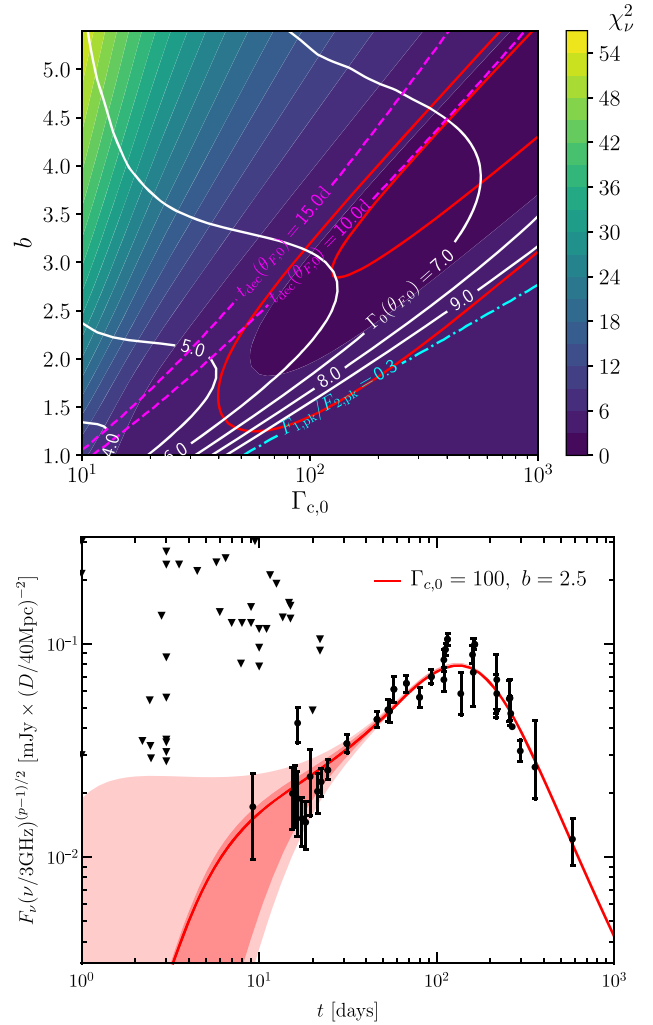
Figure 17. Top: reduced chi-square ( \chi^2_{\nu} ) contour map obtained by fitting the PL model of GG18 (with the same a , \theta_c , \theta_{\text{obs}} as in Fig. 15) to the afterglow data of GRB 170817A. The outer and inner solid red curves encompass regions in the parameter space that give the best-fitting solution with \chi^2_{\nu} \leq 3.2 and \leq 2.7 , respectively. These regions are constrained from above by dashed magenta lines for which the parameter space below the lines always yield the condition that t_{\text{dec}}(\theta_{\text{F},0}) < t_1 , where t_1 are representative times of the early afterglow observations. Another constraint is shown by a dotted-dashed cyan line for which the region above the line always yield the flux ratio F_{1,\text{pk}}/F_{2,\text{pk}} < 0.3 . Solid white contour lines indicate the initial bulk Lorentz factor of the initial angle that dominated the flux. Bottom: PL jet model light-curve fit to the afterglow data of GRB 170817A, with upper limits marked with downward triangles. The solid red curve shows the best-fitting solution of Gill & Granot (2018) and Gill et al. (2019). The lighter and darker shaded red regions encompass light curves obtained for \{\Gamma_{c,0}, b\} values with best-fitting \chi^2_{\nu} \leq 3.2 and \leq 2.7 , respectively.
