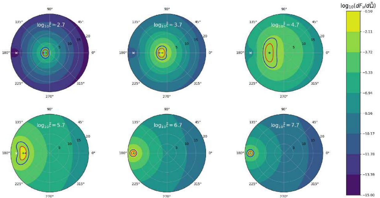
Figure 2. Angular map of dF_\nu/d\tilde{\Omega} at different times, where d\tilde{\Omega} denotes the solid angle centred around the LOS to the observer. A white cross marks the axis of the jet. The peak of dF_\nu/d\tilde{\Omega}(\tilde{t}) is \theta_{\text{obs}} - \theta_F(\tilde{t}) and is marked with a green '+' sign. Red and blue contours contain angular regions contributing 50 per cent and 80 per cent of the total flux, respectively. For comparison, we show with a blue '+' sign the value of \theta_{\text{obs}} - \theta_{\min}(\tilde{t}) . Results are plotted using the method outlined in GG18 for \Gamma_c = 1000 , \theta_c = 0.03 , a = 4 , b = 2 , \theta_{\text{obs}} = 0.3 , k = 0 , p = 2.2 , and for a frequency such that the emission is dominated by PLS G of the synchrotron emission.
