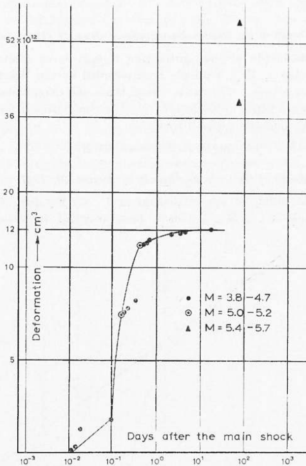
Fig. 11 - Deformation characteristics of the aftershock sequence of the Larissa Earthquake of March 1, 1941.
