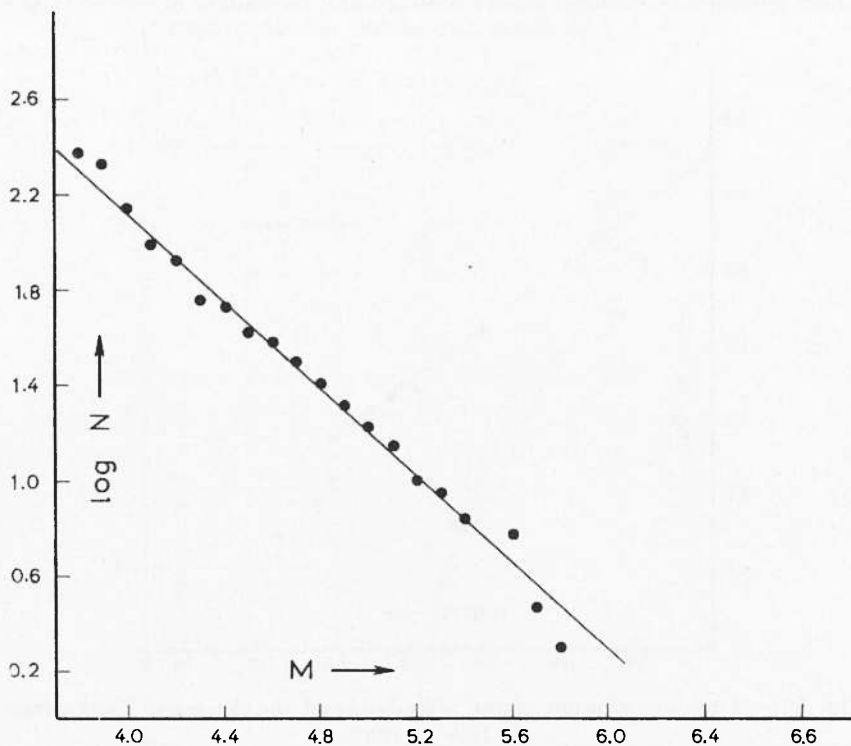
Fig. 31 - Distribution of the Magnitudes of the aftershocks of the Amorgos Earthquake of July 9, 1956.
