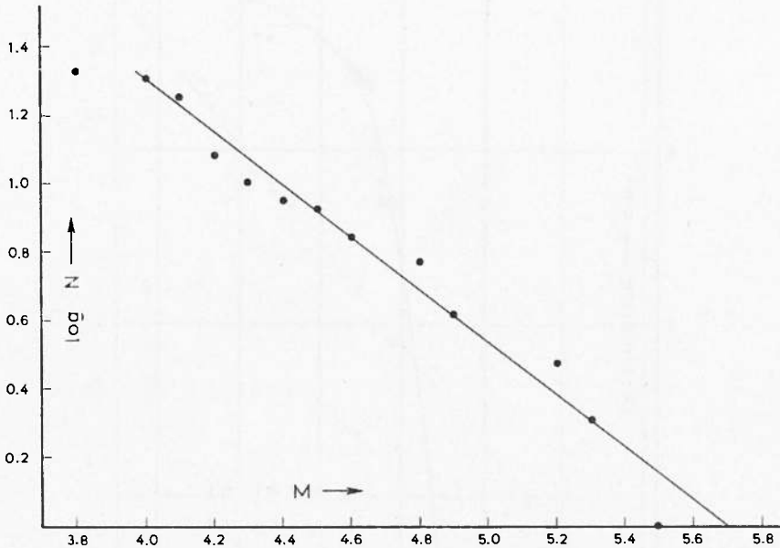
Fig. 23 - Distribution of the Magnitudes of the aftershocks of the Lemnos Earthquake of August 3, 1954.
