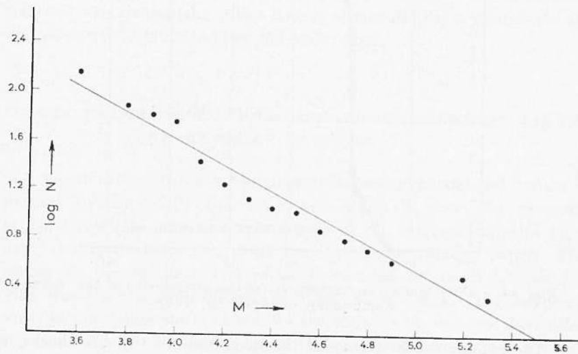
Fig. 43 - Distribution of the Magnitudes of the aftershocks of the Zante Earthquake of April 10, 1962.
