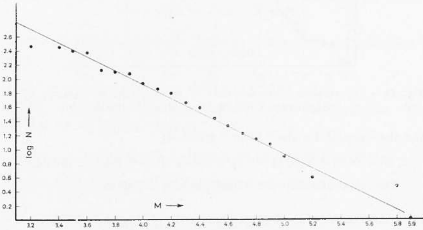
Fig. 21 - Distribution of the Magnitudes of the aftershocks of the Shophades Earthquake of April 30, 1954.
