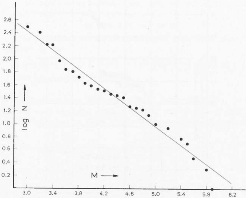
Fig. 37 - Distribution of the Magnitudes of the aftershocks of the Magnesia Earthquake of March 8, 1957.
