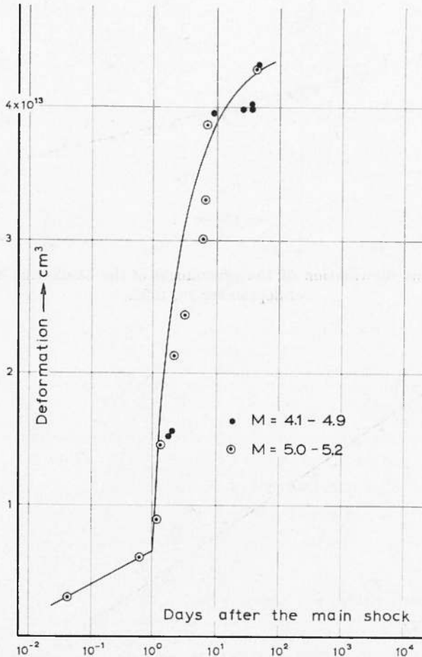
Fig. 6 - Deformation characteristics of the aftershock sequence of the Corinth Earthquake of April 22, 1928.
