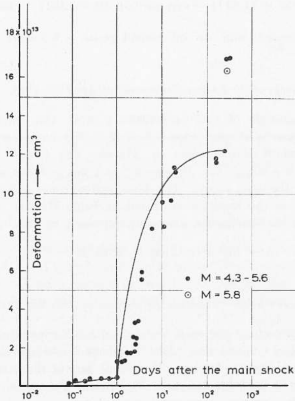
Fig. 13 - Deformation characteristics of the aftershock sequence of the Karpathos Earthquake of February 9, 1948.
