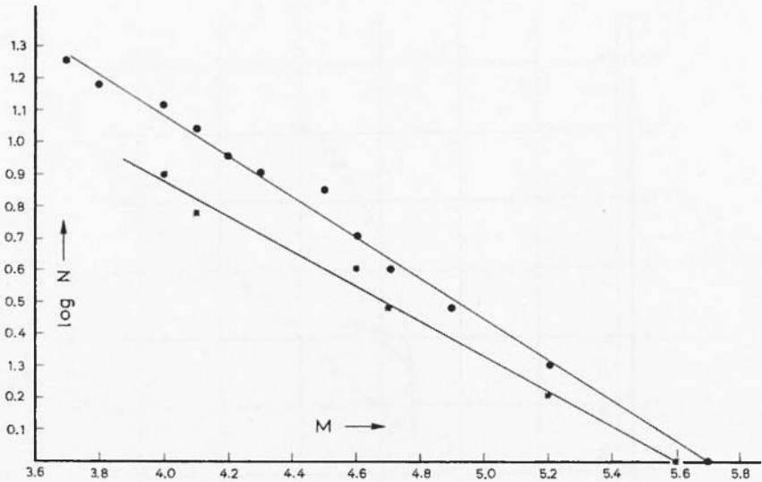
Fig. 33 - Distribution of the Magnitudes of the foreshocks and aftershocks of the NE-Crete Earthquake of July 30, 1956.
