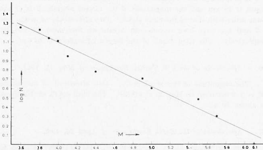
Fig. 41 - Distribution of the Magnitudes of the aftershocks of the Zante Earthquake of November 15, 1959.
