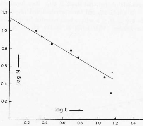
Fig. 34 - Time distribution of the aftershocks of the Messina Earthquake of February 19, 1957.
