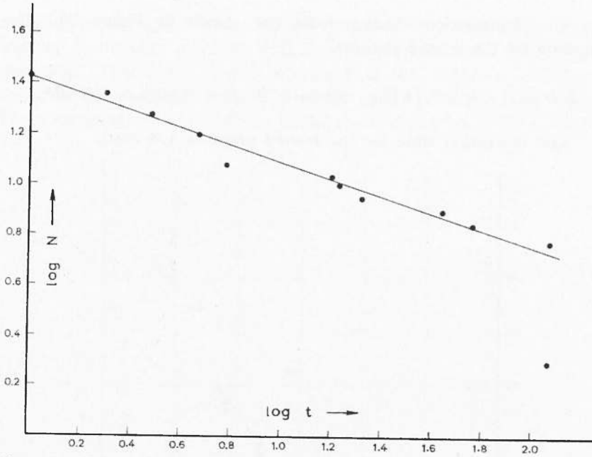
Fig. 27 - Time distribution of the aftershocks of the Samos Earthquake of July 15, 1955.
