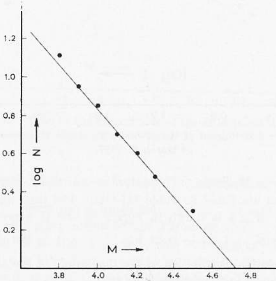
Fig. 35 - Distribution of the Magnitudes of the aftershocks of the Messina Earthquake of February 19, 1957.
