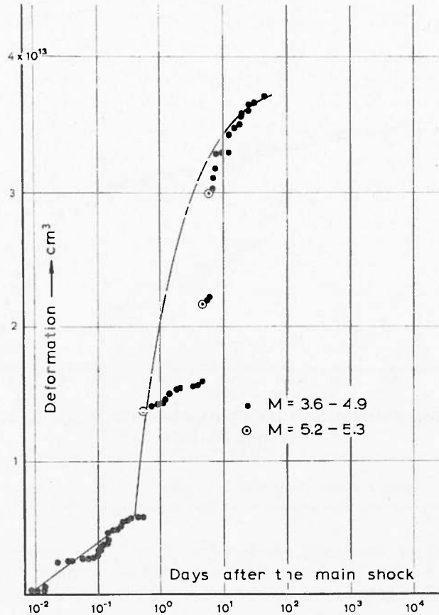
Fig. 22 - Deformation characteristics of the aftershock sequence of the Shophades Earthquake of April 30, 1954.
