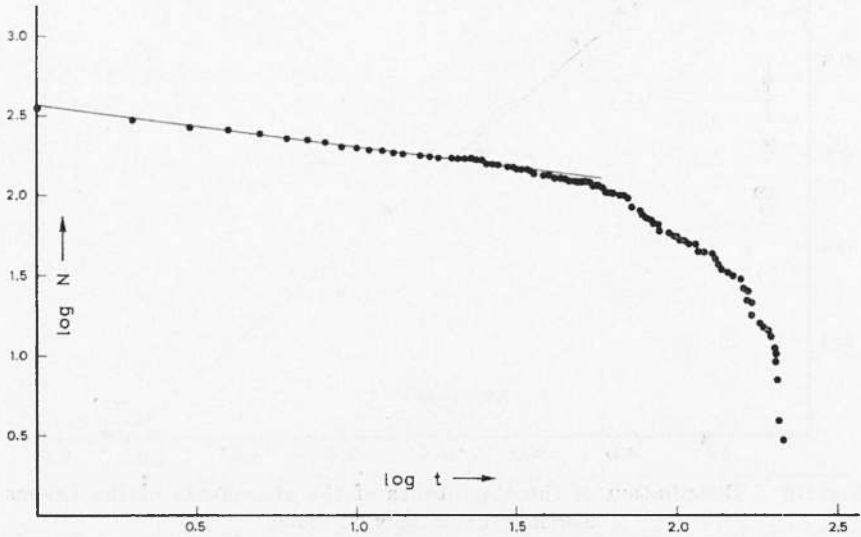
Fig. 17 - Time distribution of the aftershocks of the Kephallenia Earthquake of August 12, 1953.
