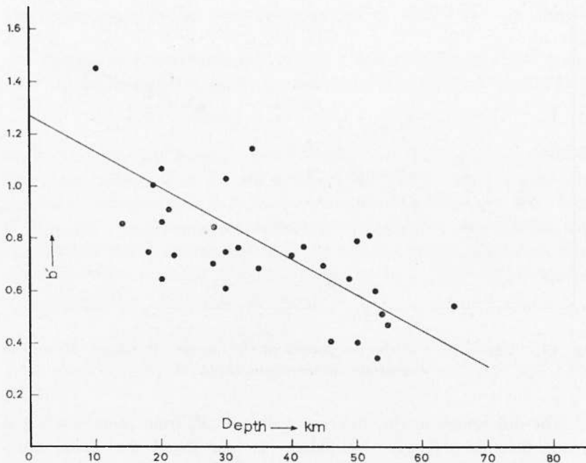
Fig. 46 - Dependence of the constant b' of the cumulative frequency function of the magnitude on the focal depth.
