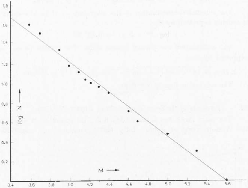
Fig. 40 - Distribution of the Magnitudes of the aftershocks of the Zante Earthquake of August 27, 1958.
