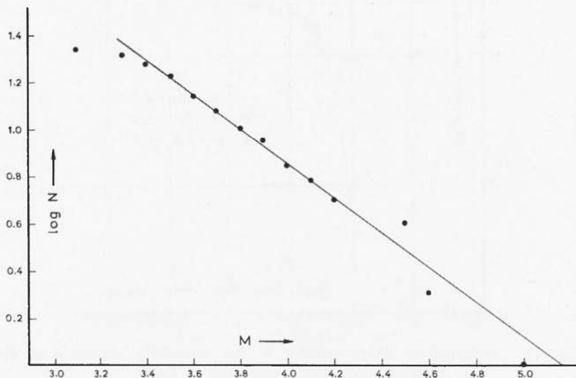
Fig. 12 - Distribution of the Magnitudes of the aftershocks of the Crete Earthquake of August 30, 1947.
