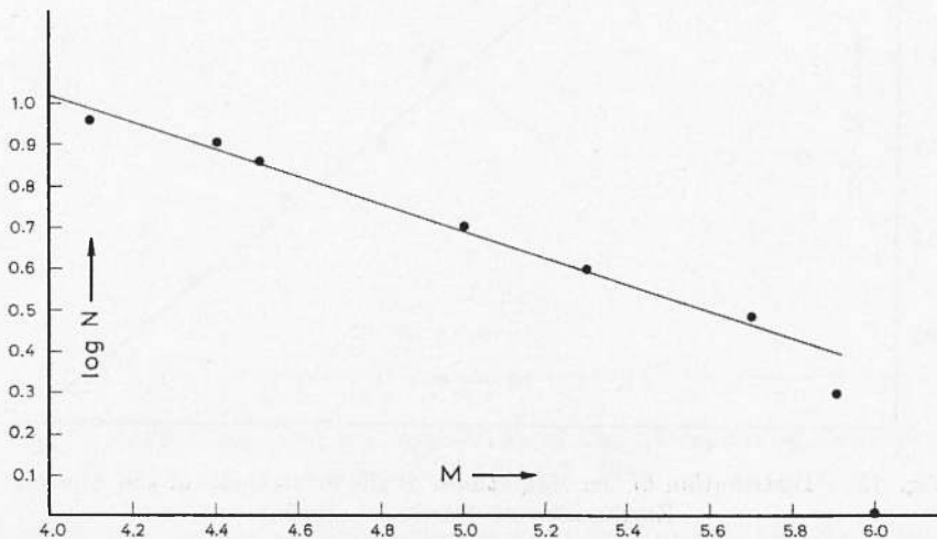
Fig. 14 - Distribution of the Magnitudes of the aftershocks of the SW Crete Earthquake of December 17, 1952.
