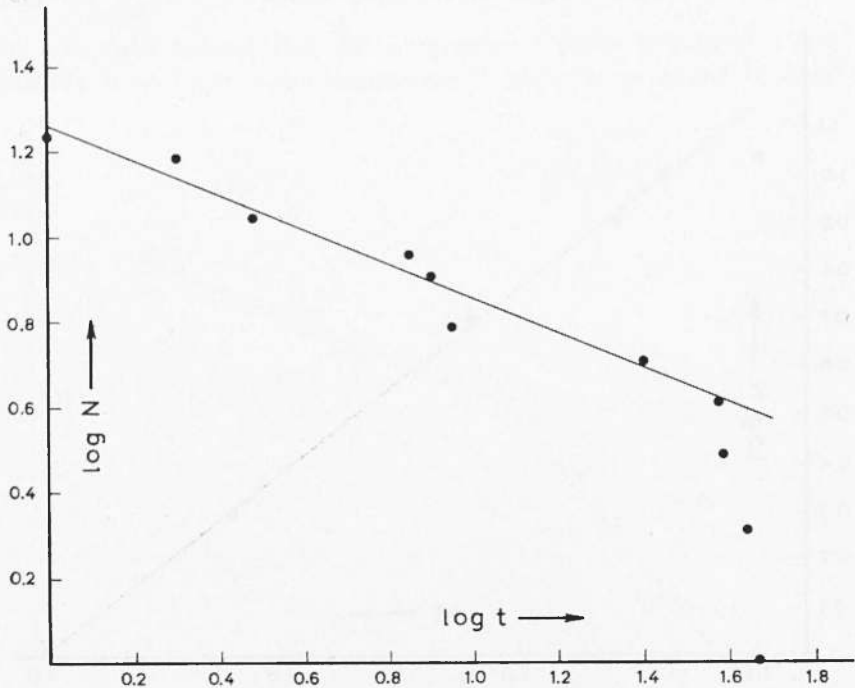
Fig. 5 - Time distribution of the aftershocks of the Corinth Earthquake of April 22, 1928.
