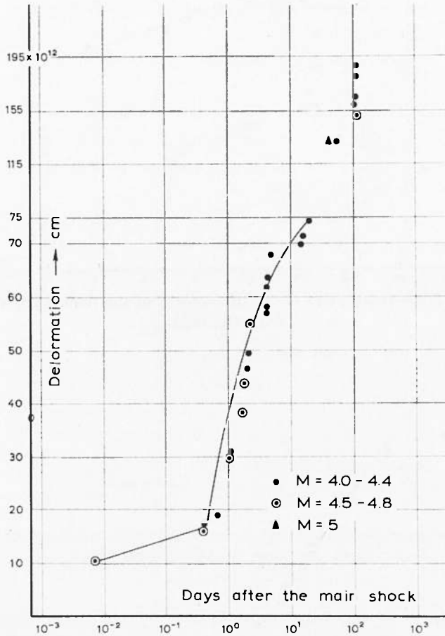
Fig. 29 - Deformation characteristics of the aftershock sequence of the Samos Earthquake of July 15, 1955.
