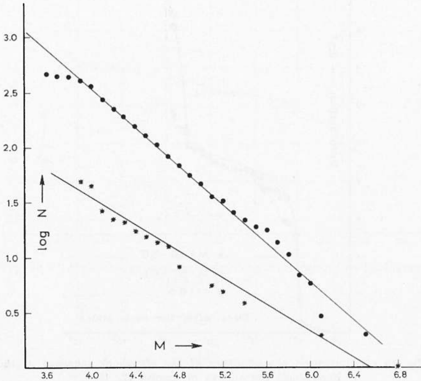
Fig. 18 - Distribution of the Magnitudes of the aftershocks and foreshocks of the Kephallenia Earthquake of August 12, 1953.
