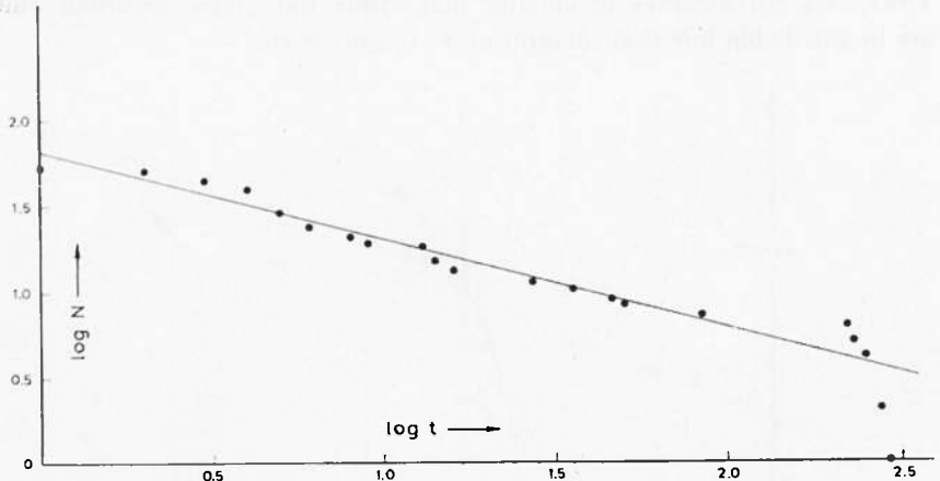
Fig. 7 - Time distribution of the aftershocks of the Chalkidike Earthquake of September 26, 1932.
