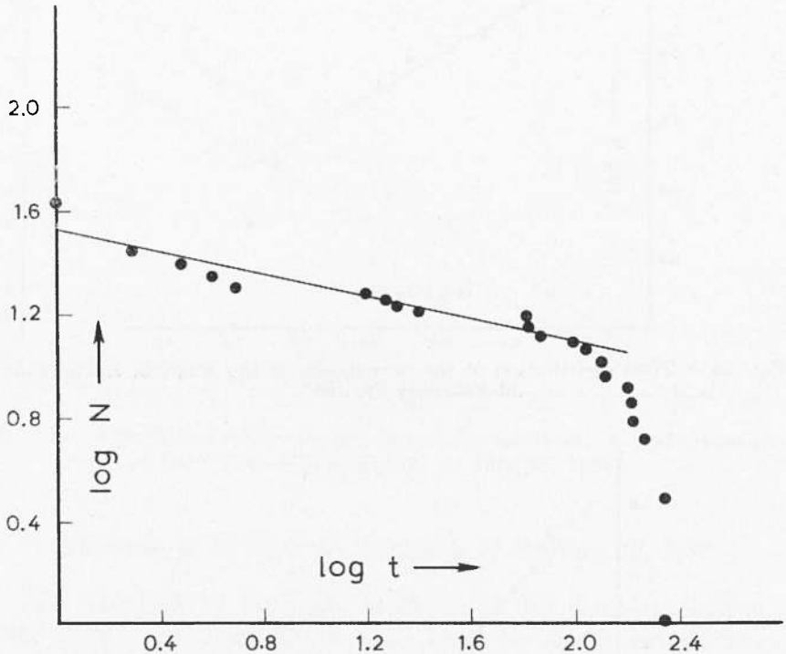
Fig. 36 - Time distribution of the aftershocks of the Magnesia Earthquake of March 8, 1957.
