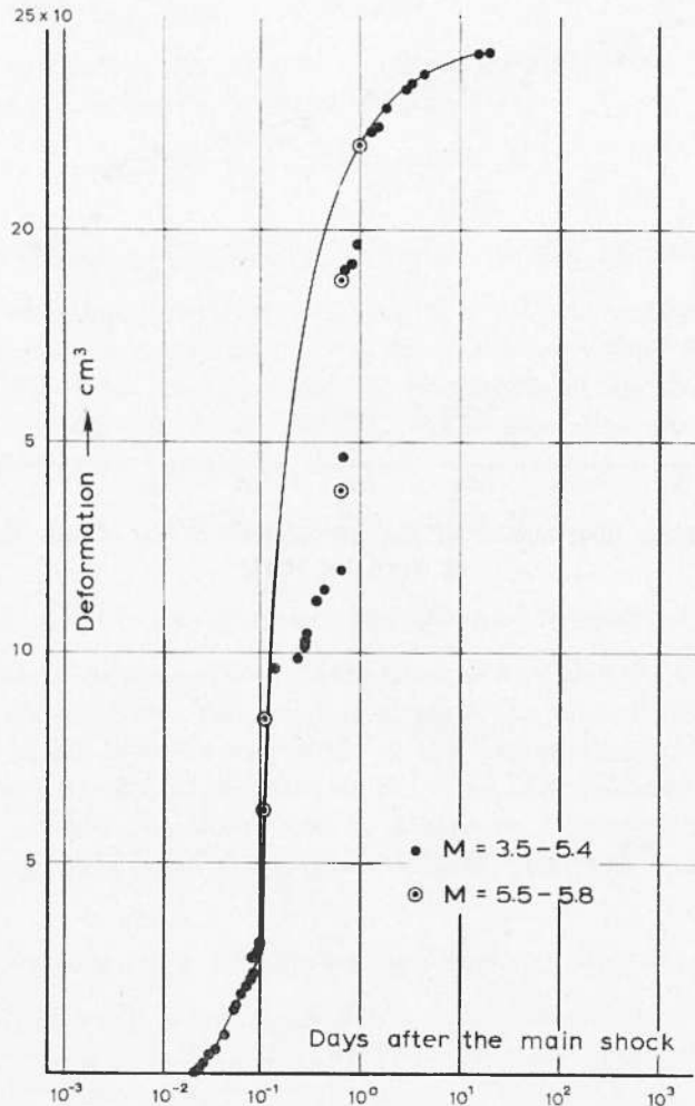
Fig. 44 - Deformation characteristics of the aftershocks of the Zante Earthquake of April 10, 1962.
