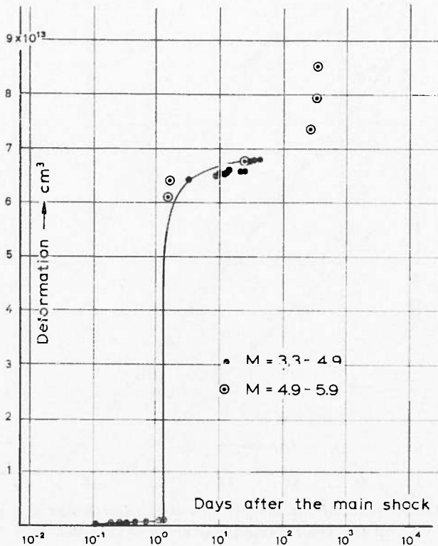
Fig. 26 - Deformation characteristics of the aftershock sequence of the Volos Earthquake of April 19, 1955.
