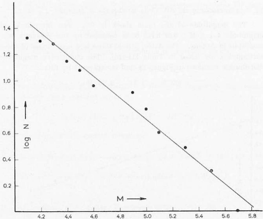
Fig. 15 - Distribution of the Magnitudes of the aftershocks of the Anatolia Earthquake of March 18, 1953.
