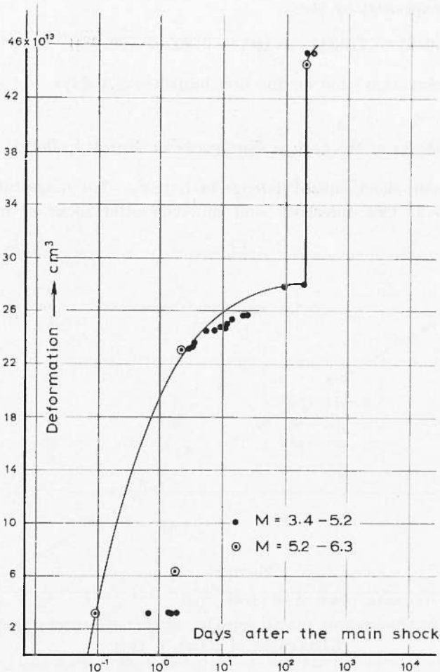
Fig. 9 - Deformation characteristics of the aftershock sequence of the Chalkidike Earthquake of September 26, 1932.
