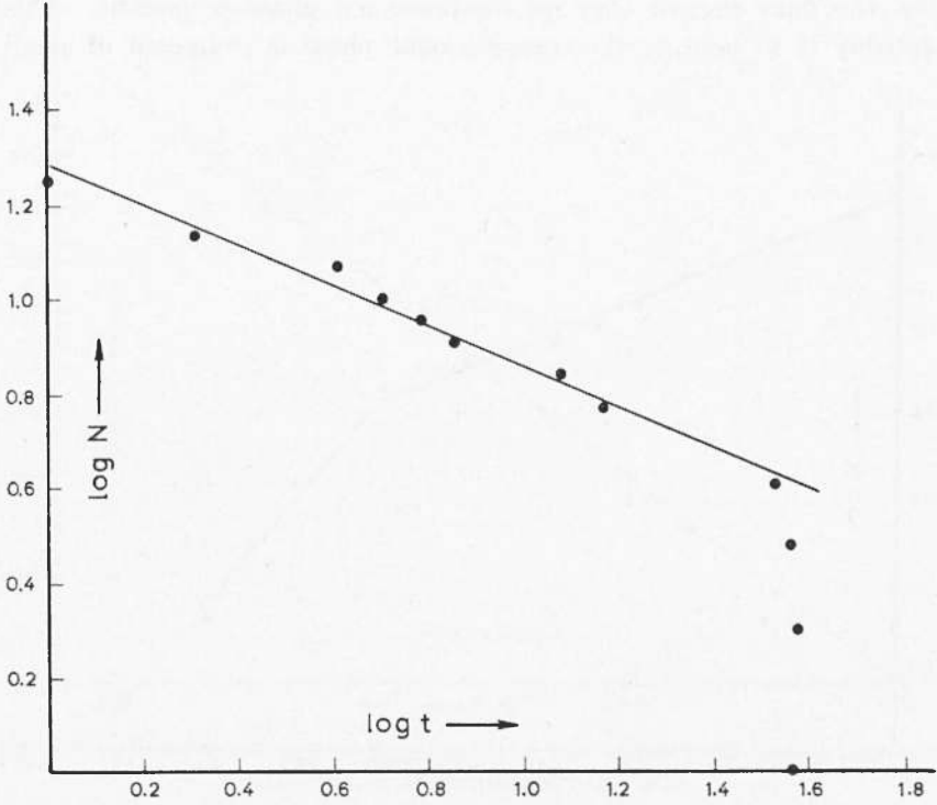
Fig. 2 - Time distribution of the aftershocks of the Southern Sporades Earthquake of March 18, 1926.
