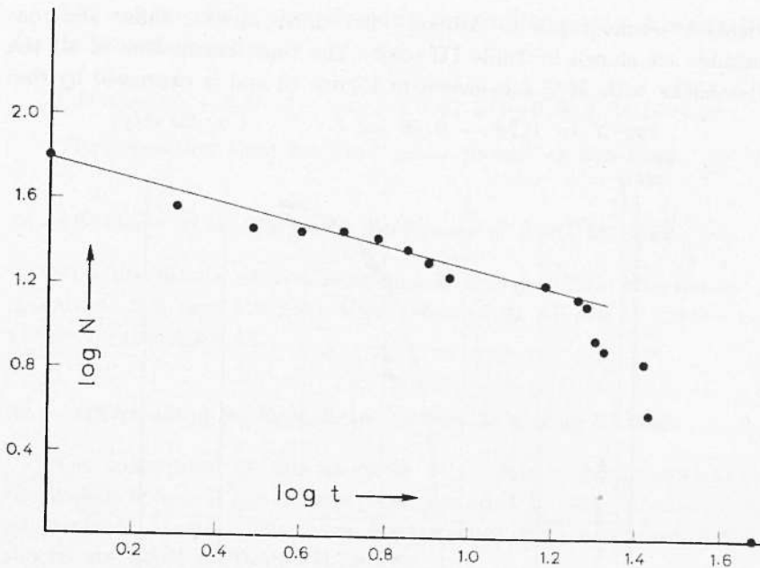
Fig. 42 - Time distribution of the aftershocks of the Zante Earthquake of April 10, 1962.
