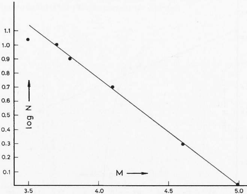
Fig. 4 -- Distribution of the Magnitudes of the aftershocks of the Messina Earthquake of September 19, 1926.
