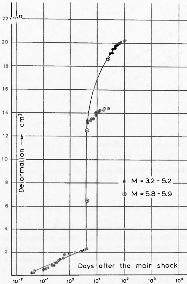
Fig. 32 - Deformation characteristics of the aftershock sequence of the Amorgos Earthquake of July 9, 1956.
