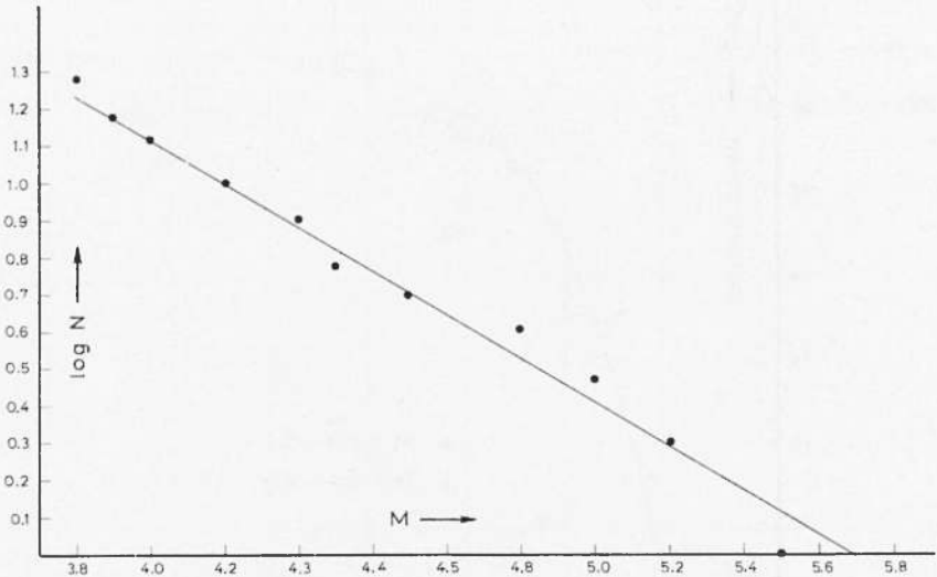
Fig. 10 - Distribution of the Magnitudes of the aftershocks of the Larissa Earthquake of March 1, 1941.
