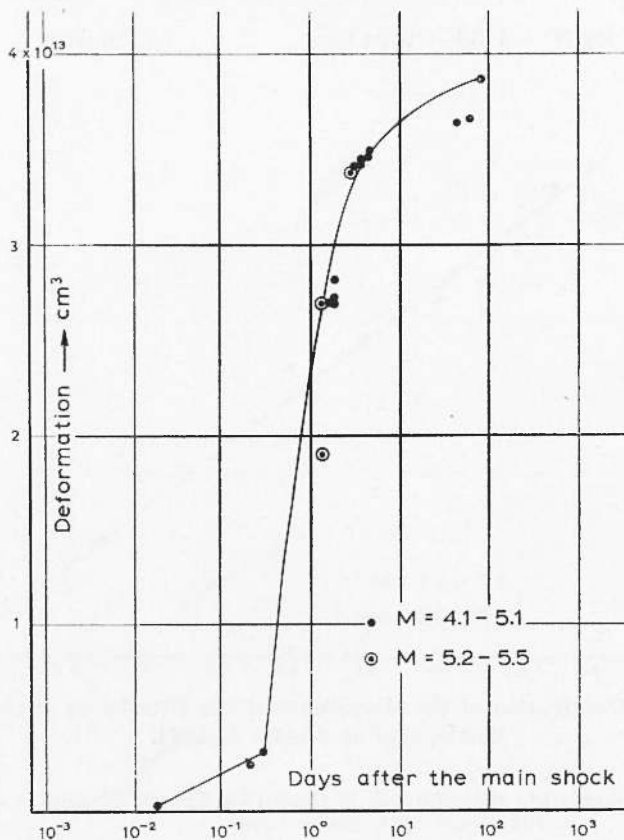
Fig. 24 - Deformation characteristic of the aftershock sequence of the Lemnos Earthquake of August 3, 1954.
