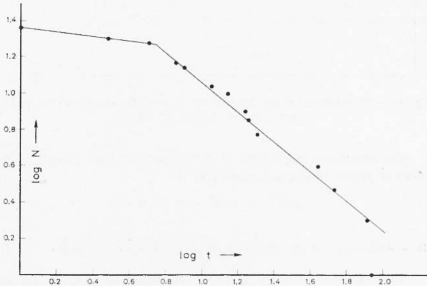
Fig. 39 - Time distribution of the aftershocks of the Zante Earthquake of August 27, 1958.
