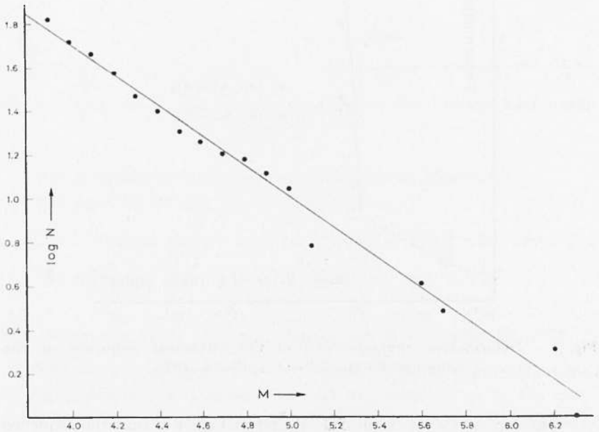
Fig. 8 - Distribution of the Magnitudes of the aftershocks of the Chalkidike Earthquake of September 26, 1932.
