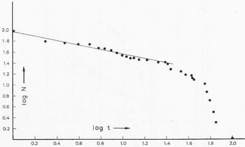
Fig. 20 - Time distribution of the aftershocks of the Shophades Earthquake of April 30, 1954.
