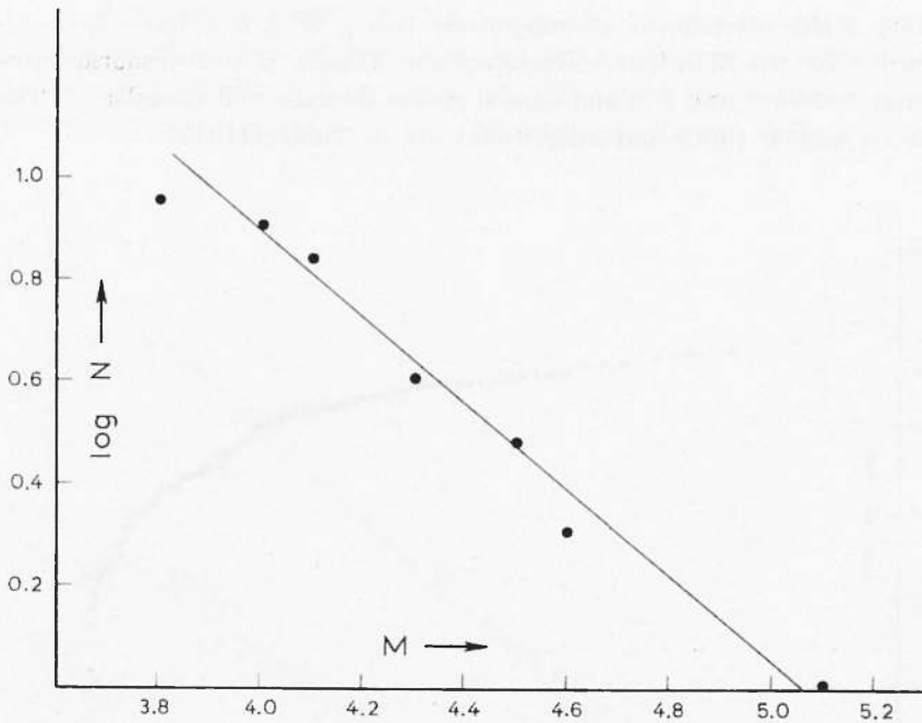
Fig. 16 - Distribution of the Magnitudes of the aftershocks of the Lesbos Earthquake of May 2, 1953.
