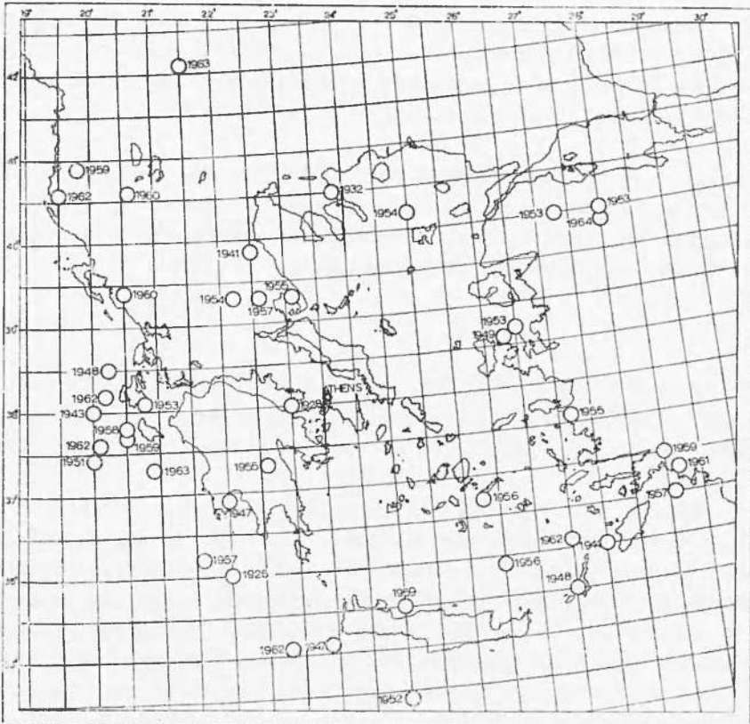
Fig. 1 - Index map of the epicenters of the shallow earthquakes of M \geq 6 occurred in the region of Greece from 1926 till 1964.
