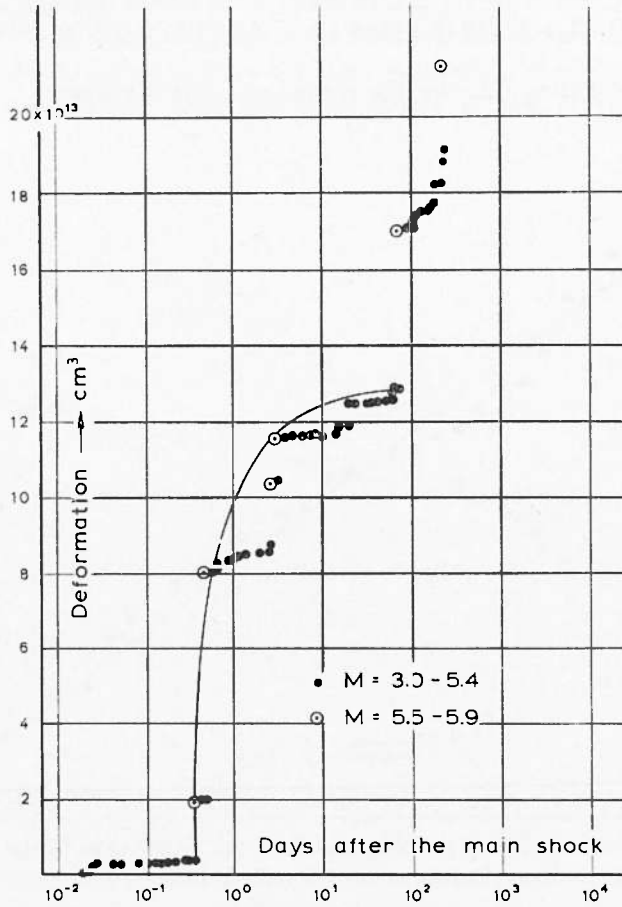
Fig. 38 - Deformation characteristics of the aftershock sequences of the Magnesia Earthquake of March 8, 1957.
