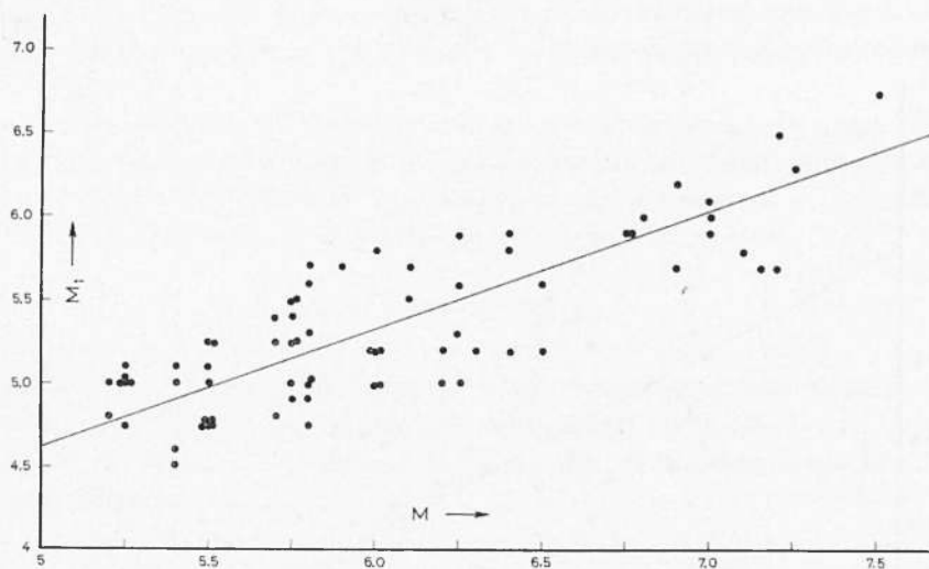
Fig. 45 - Dependence of the magnitude of the largest aftershock M_1 on the Magnitude of the main shock M .
