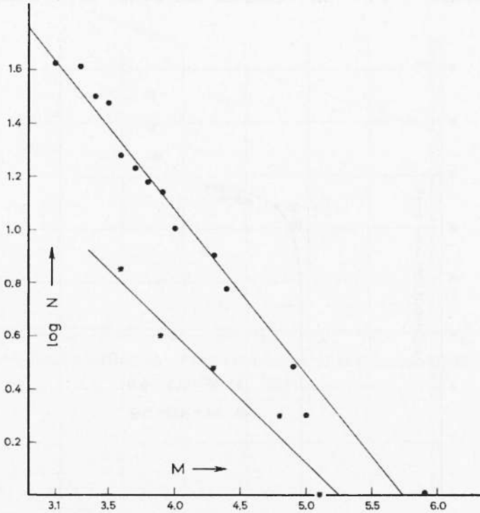
Fig. 25 - Distribution of the Magnitudes of the foreshocks and aftershocks of the Volos Earthquake of April 19, 1955.
