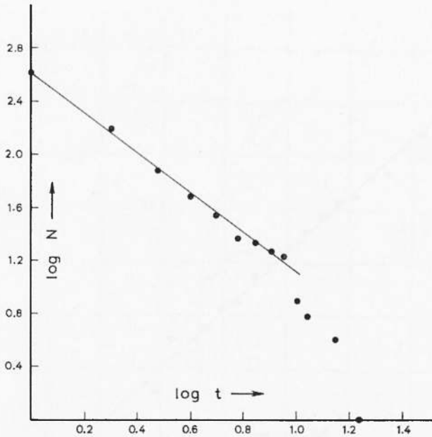
Fig. 30 - Time distribution of the aftershocks of the Amorgos Earthquake of July 9, 1956.
