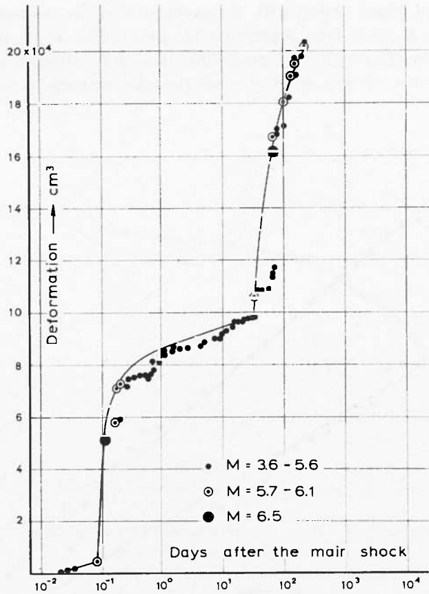
Fig. 19 - Deformation characteristics of the aftershock sequence of the Kephallenia Earthquake of August 12, 1953.
