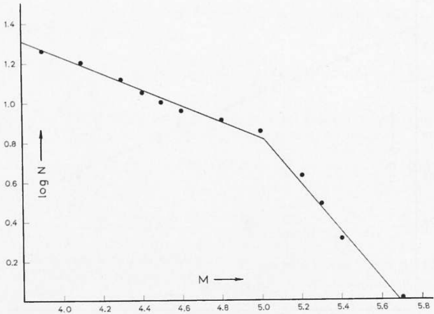
Fig. 3 - Distribution of the Magnitudes of the aftershocks of the Southern Sporades Earthquake of March 18, 1926.
