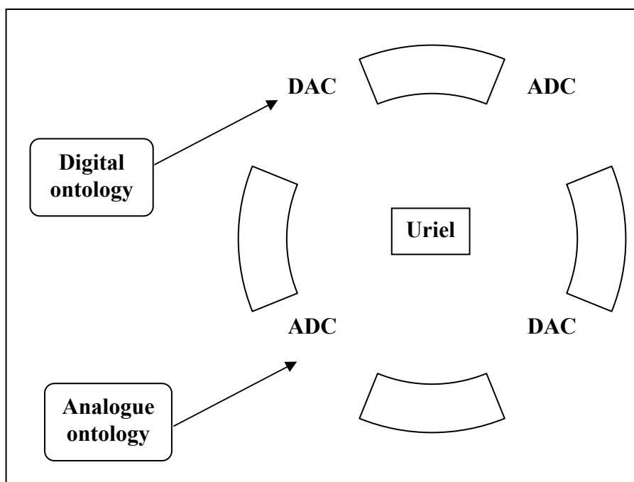
Figure 4 Fourth stage of the thought experiment, Uriel's wheel.
