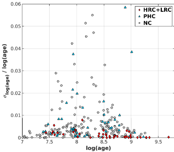
Fig. 5. BASE-9 relative error on \log(\text{age}) against \log(\text{age}) .
