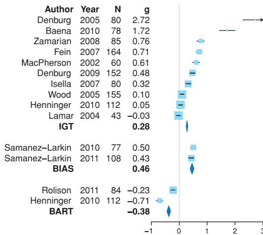
Figure 1. Decisions from experience. Forest plot for studies using decisions from experience paradigms. The positions of the squares on the x-axis indicate the effect size for each study; the bars indicate the 95% CI of the effect sizes, and the sizes of the squares are inversely proportional to the respective standard errors (i.e., larger squares indicate smaller standard errors).
