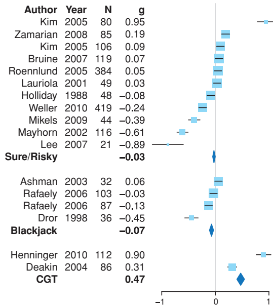
Figure 2. Decisions from description. Forest plot for studies using decisions from description paradigms. The positions of the squares on the x-axis indicate the effect size for each study; the bars indicate the 95% confidence intervals of the effect sizes, and the sizes of the squares are inversely proportional to the respective standard errors (i.e., larger squares indicate smaller standard errors).
