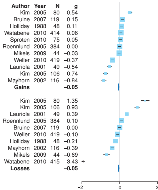
Figure 3. Decisions from description: gains vs. losses. Forest plot for studies using decisions from description and that distinguish between gain and loss domains. The positions of the squares on the x-axis indicate the effect size for each study; the bars indicate the 95% confidence intervals of the effect sizes, and the sizes of the squares are inversely proportional to the respective standard errors (i.e., larger squares indicate smaller standard errors).
