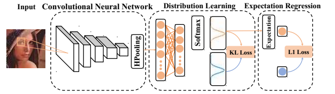
Figure 2: The framework of our DLDL-v2. Given an input image and its ground-truth age, we firstly generate a label distribution and then jointly optimize label distribution learning and expectation regression in one unified framework in an end-to-end manner.
