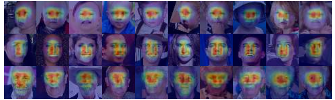
Figure 4: Examples of the score map visualizations on ChaLearn16 testing images. The first row is for infants ( [0, 3] ), the second row is for adults ( [20, 35] ) and the third row is for senior people ( [65, 100] ) (Best viewed in color and zoomed in).
